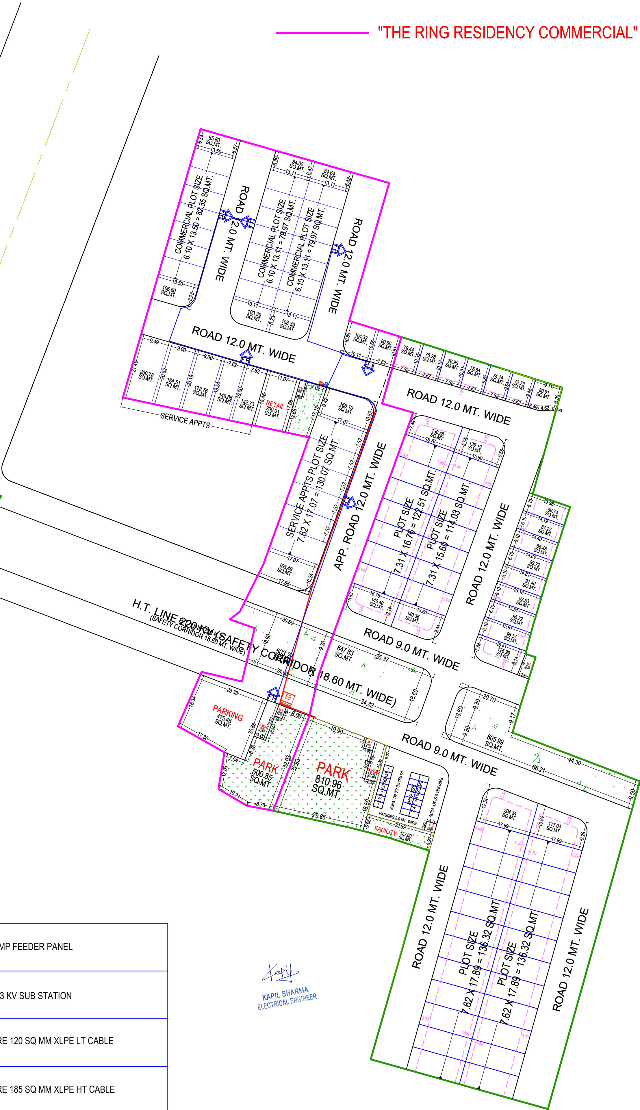
ELECTRICAL PLAN LAYOUT
