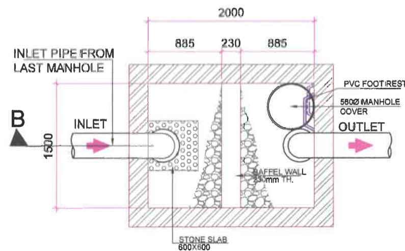
PLAN OF DESILTING CHAMBER & RWH PIT
