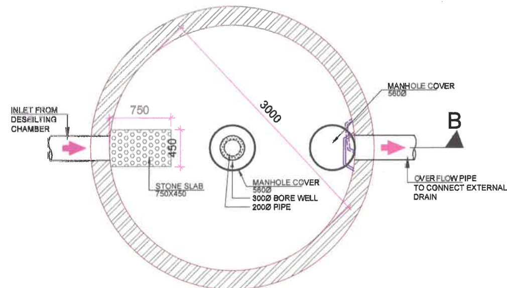
PLAN OF DESILTING CHAMBER & RWH PIT
