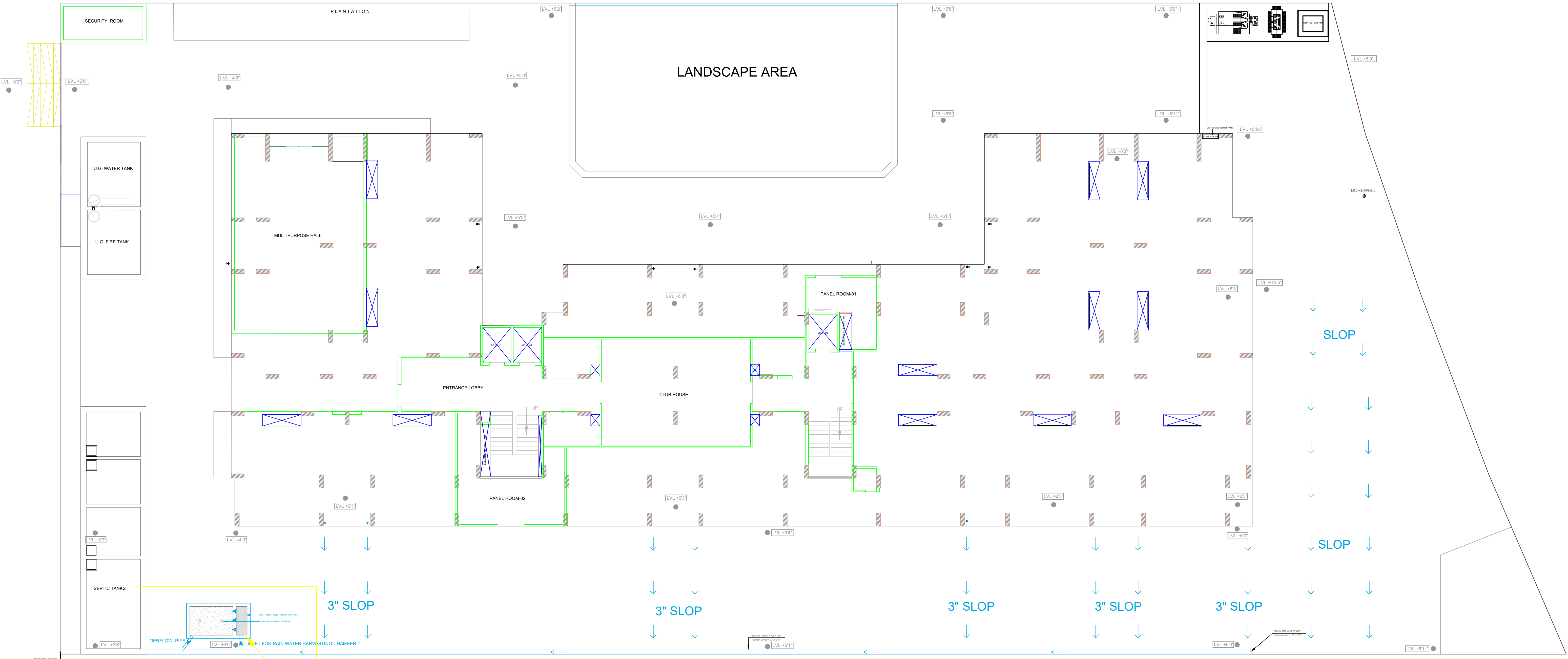
STILT FLOOR PLAN (RAIN WATER HARVESTING)
