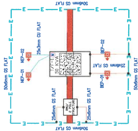
Detail-A Switch Yard Layout Plan
