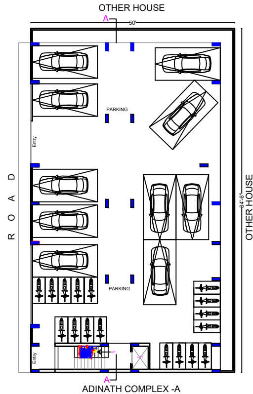
PLAN : GROUND FLOOR
