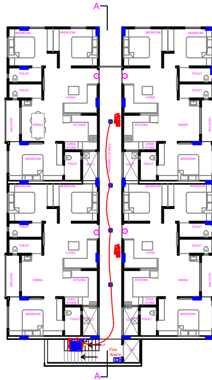
PLAN : TYPICAL FLOOR
