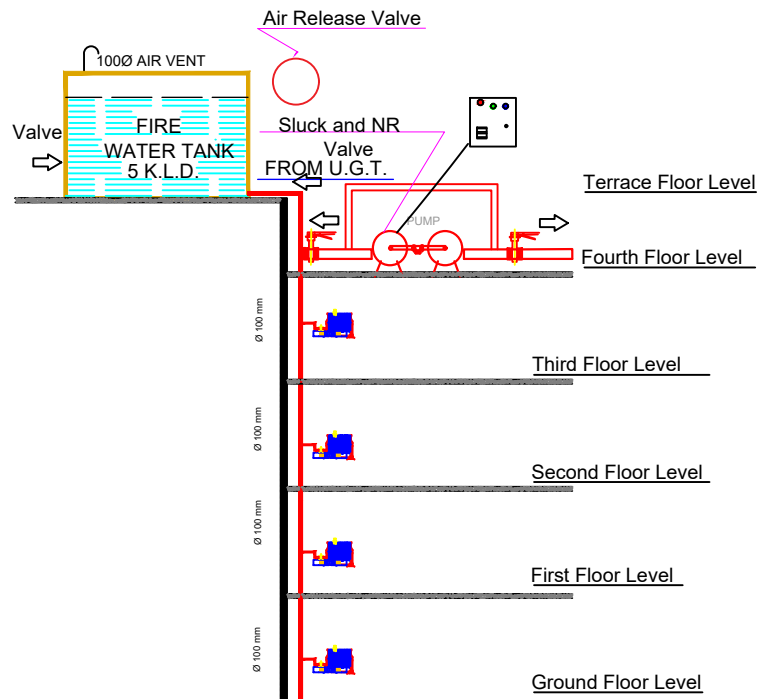
S.L.D. FIRE FIGHTING PLAN
