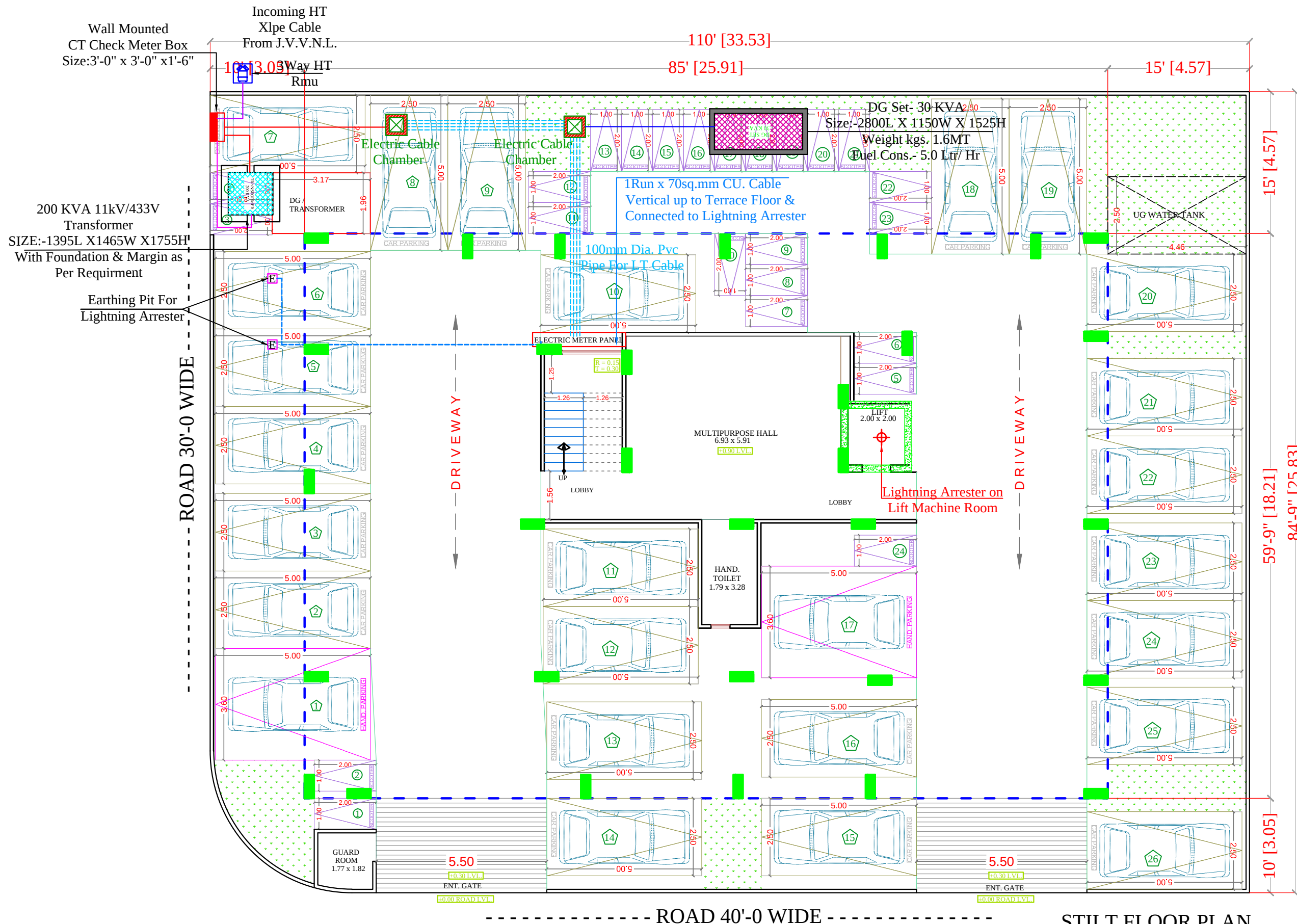
STILT FLOOR PLAN
