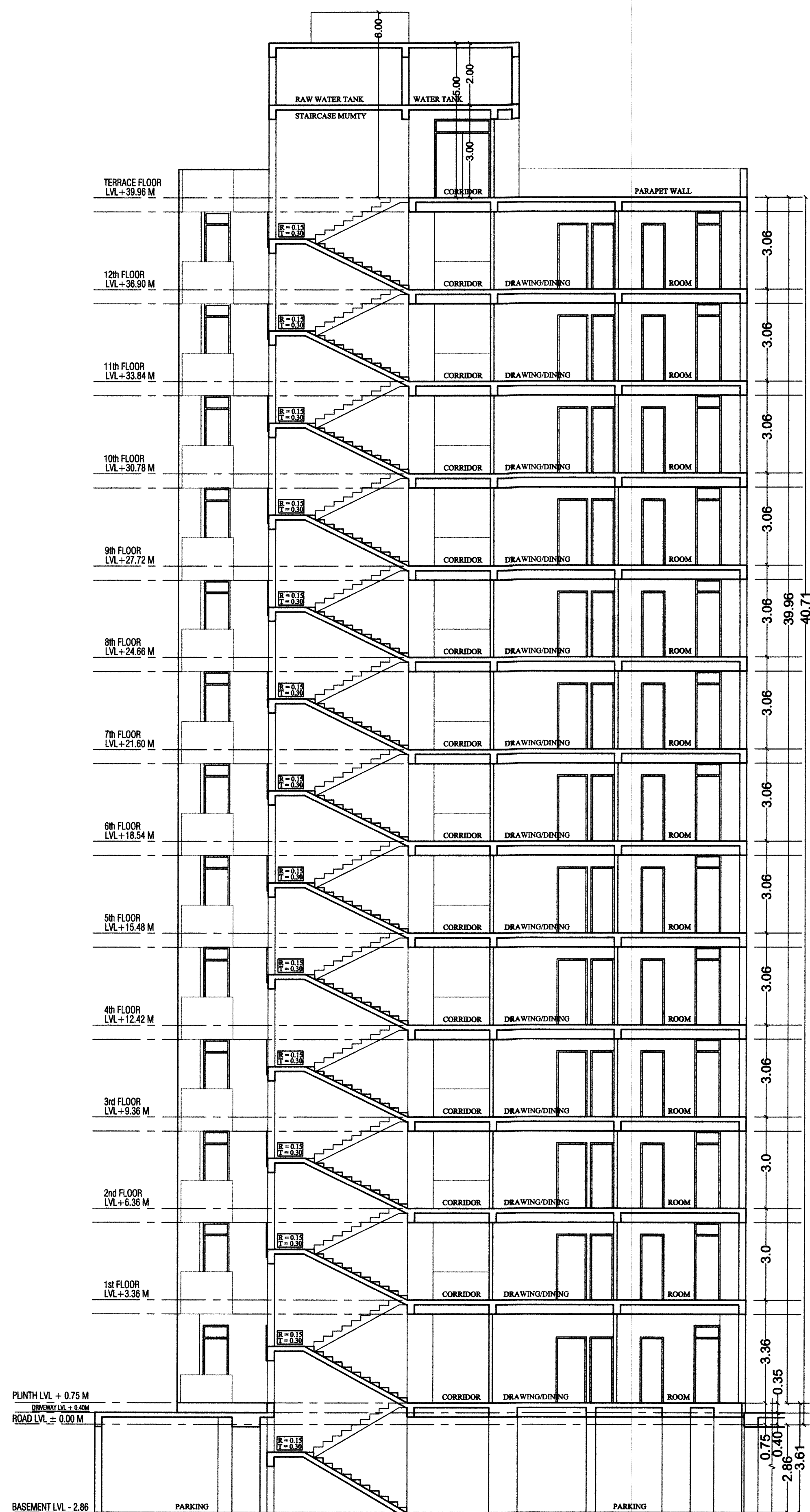
SECTION AT S1-S1
