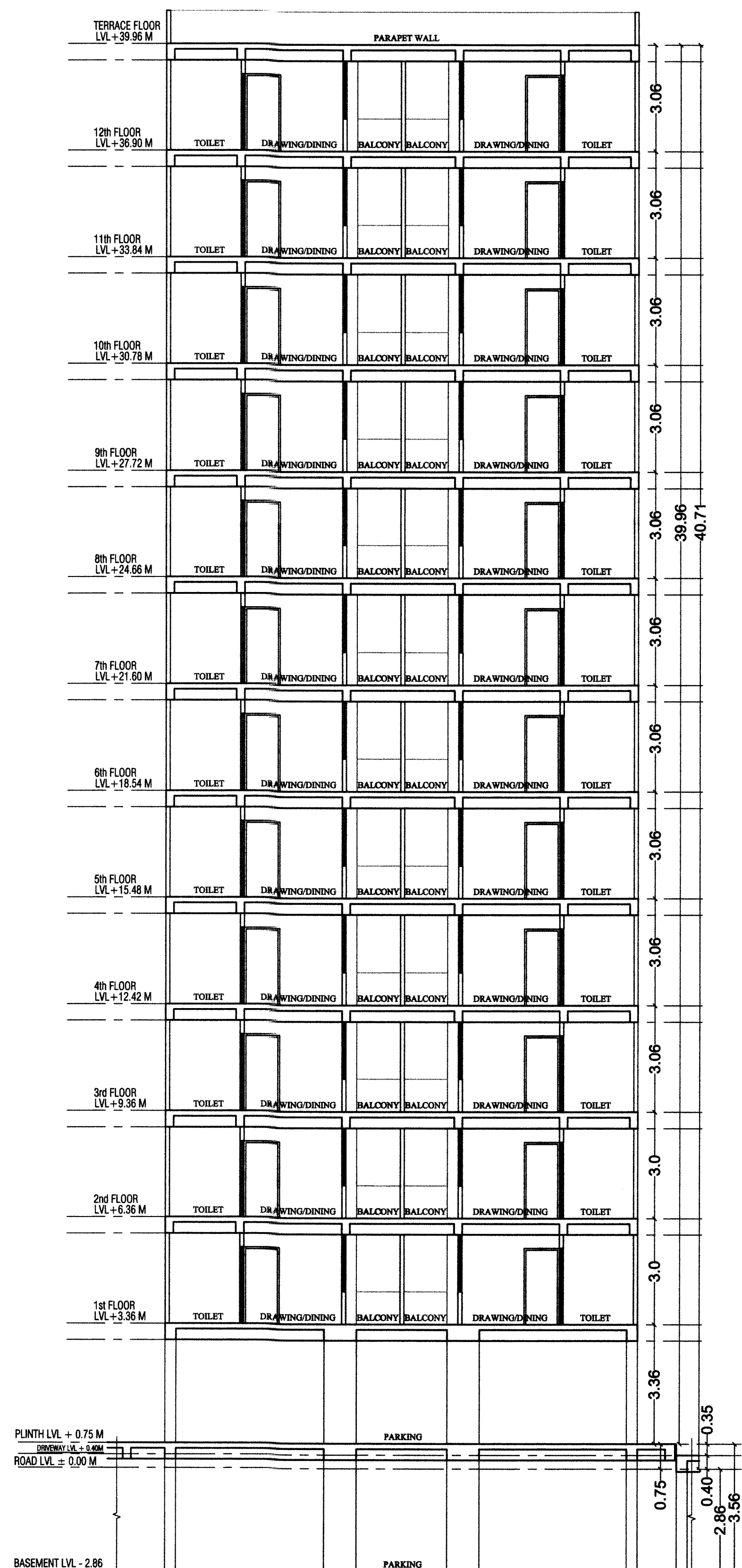
SECTION AT S2-S2
