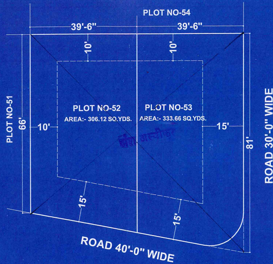
SITE PLAN
