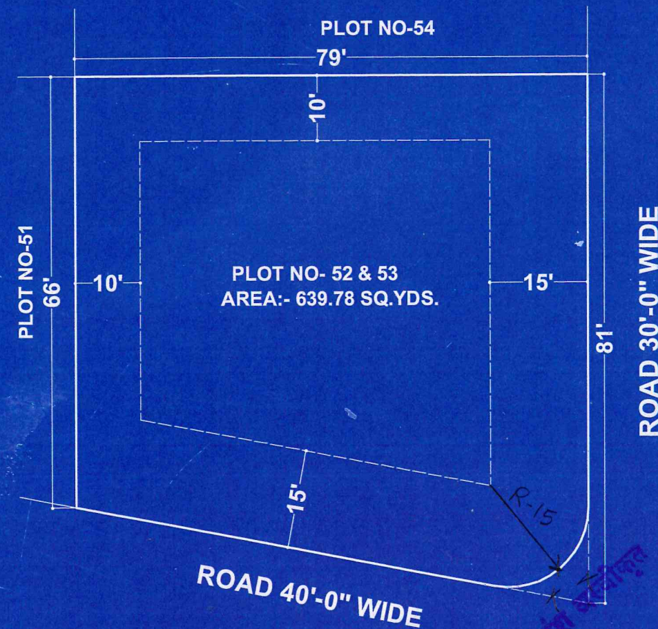
RECONSTITUTE PLAN
