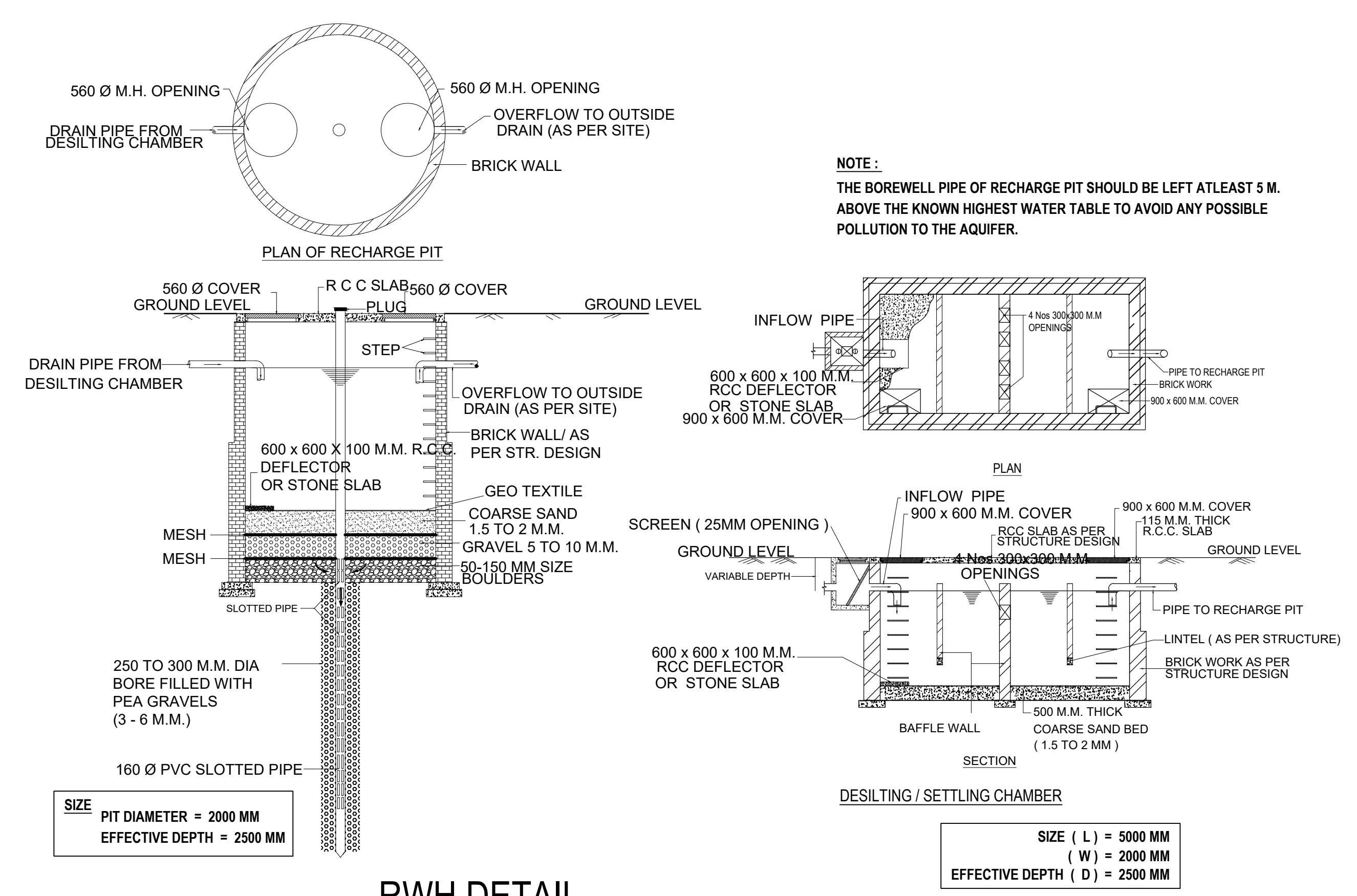
RWH DETAIL
