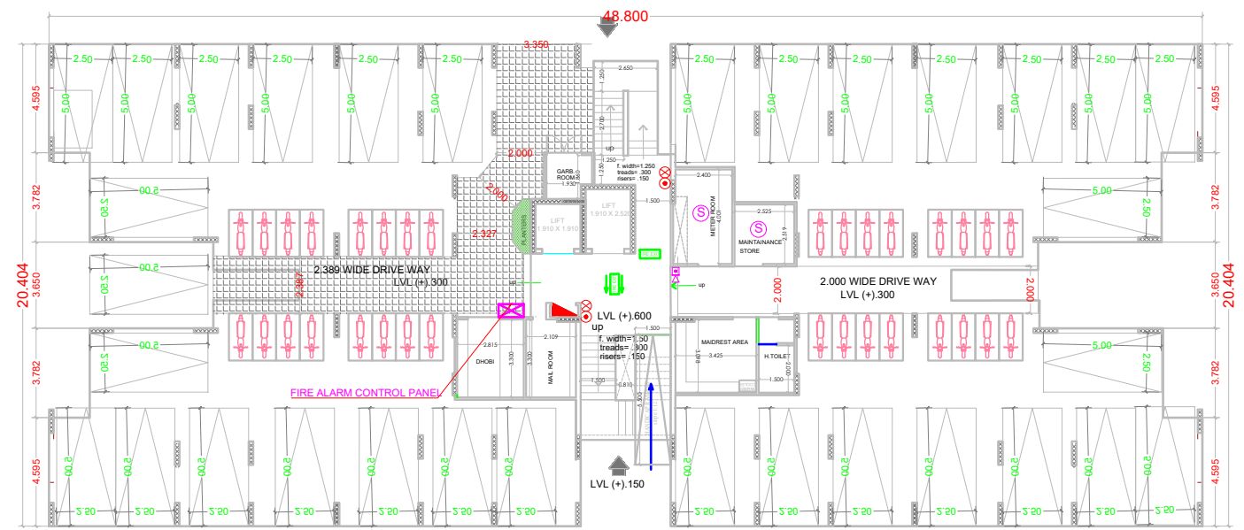
STILT FLOOR PLAN (BLOCKS 2 &amp; 5)
