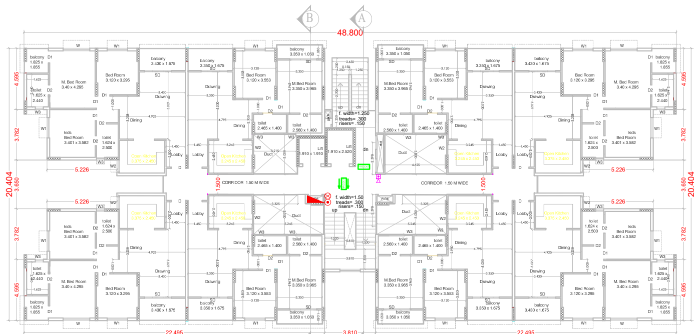
TYPICAL FLOOR PLAN (BLOCKS 1, 2, 3, 4 &amp; 5)
