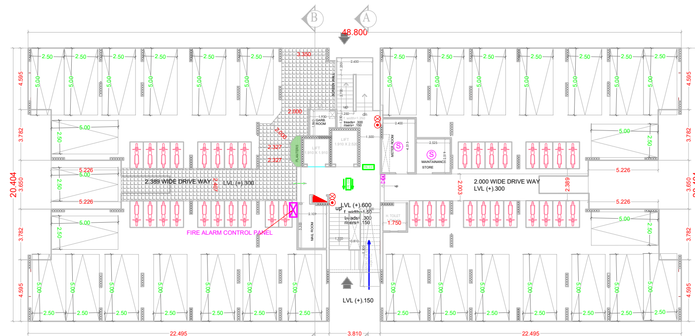
STILT FLOOR PLAN (BLOCKS 1, 3 &amp; 4)
