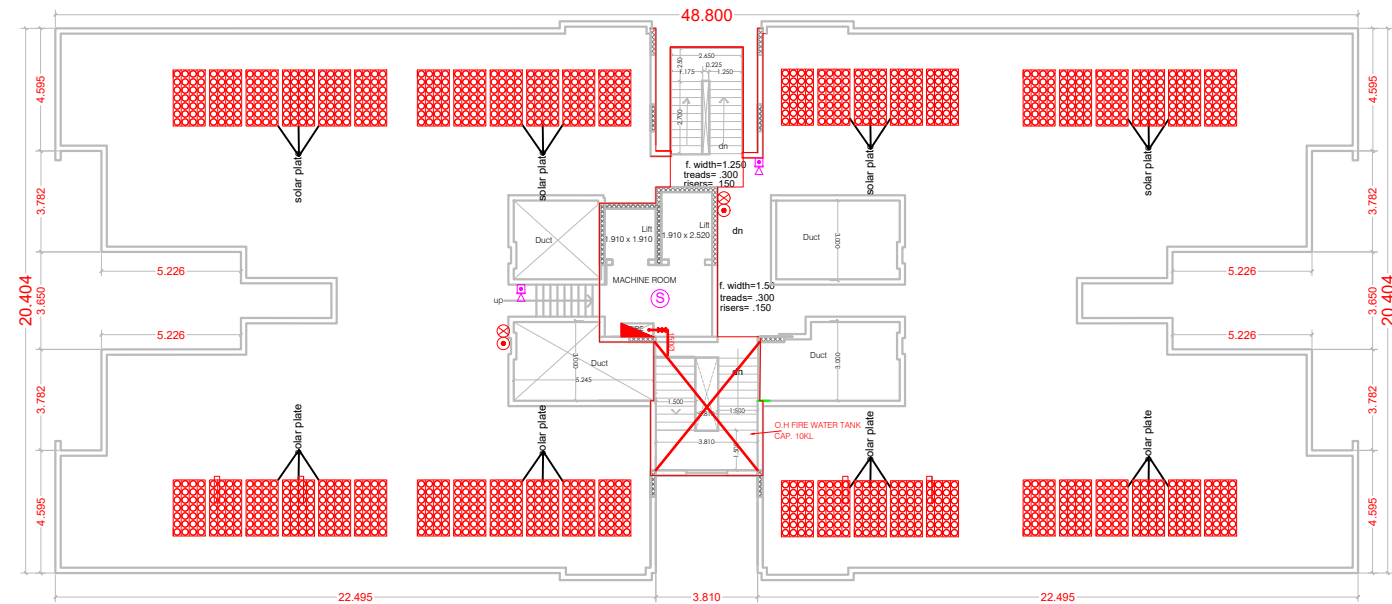
TERRACE FLOOR PLAN (BLOCKS 1, 2, 3, 4 &amp; 5)
