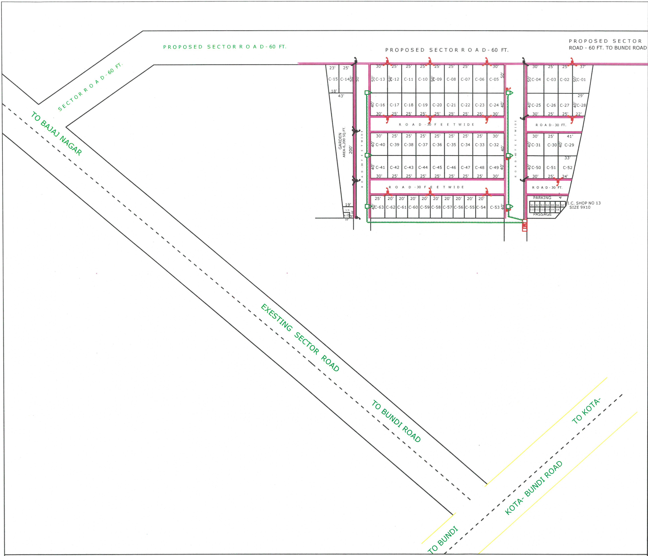
ELECTRICAL LAYOUT PLAN
