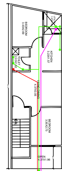
GROUND FLOOR PLAN
