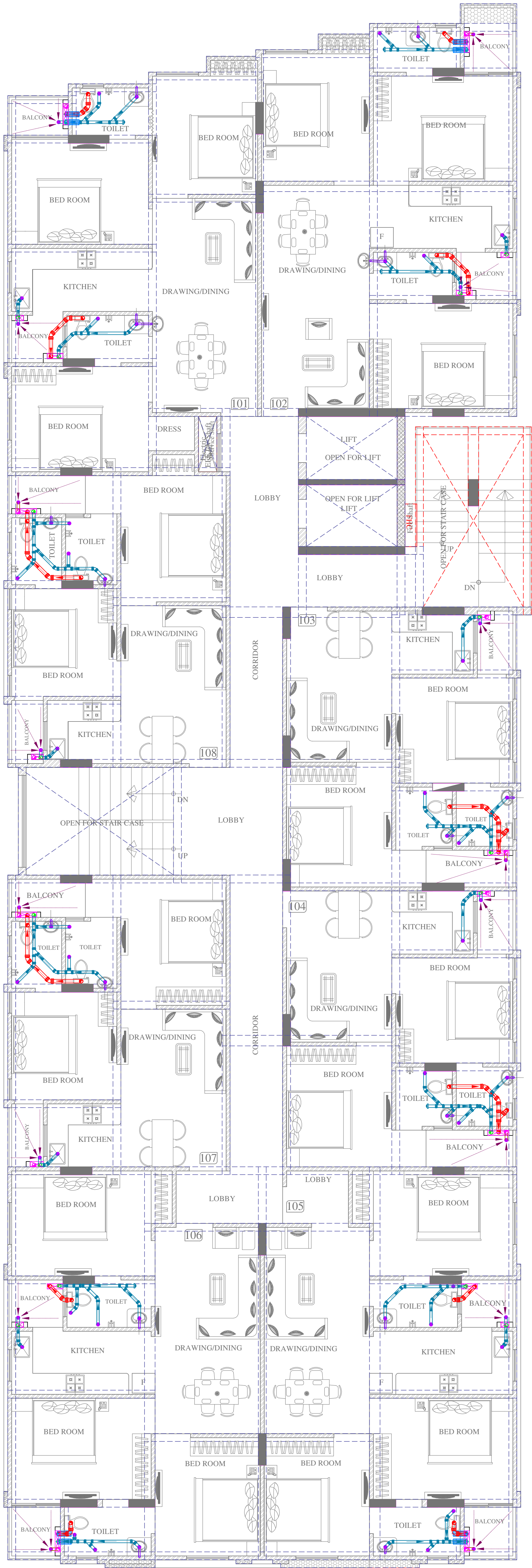
TYPICAL FLOOR INTERNAL DRAINAGE PLAN
