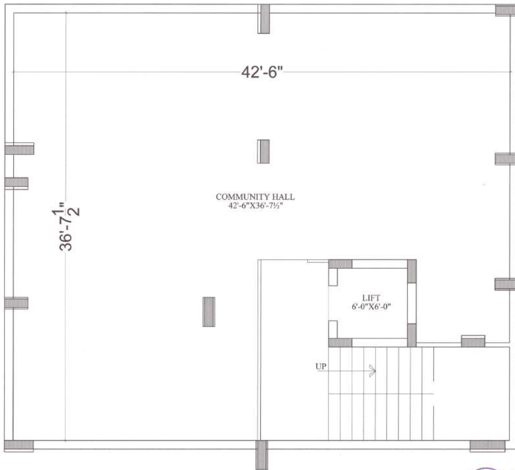
BASEMENT FLOOR WORKING PLAN
