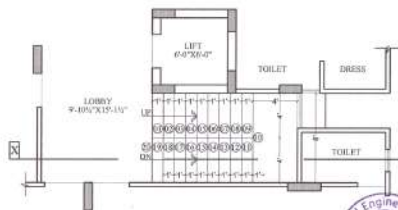
TYPICAL FLOOR PLAN
