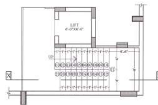
BASEMENT FLOOR PLAN
