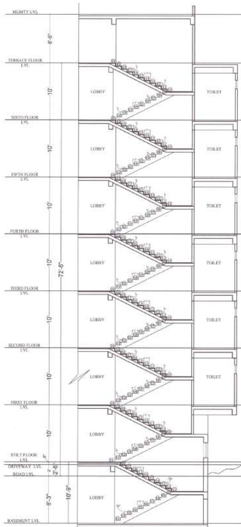
SECTION-XX
