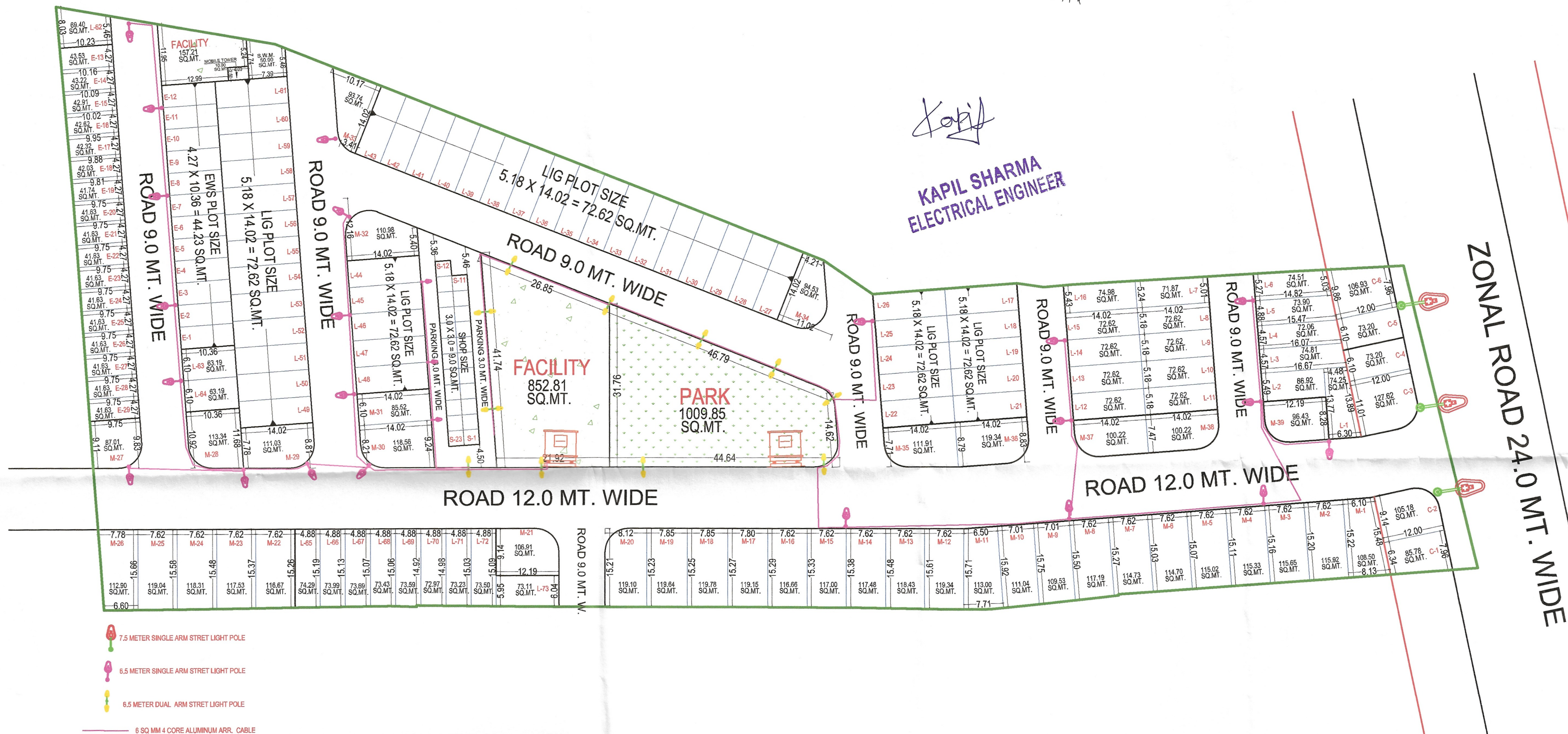
"STREET LIGHT PLAN LAYOUT"
