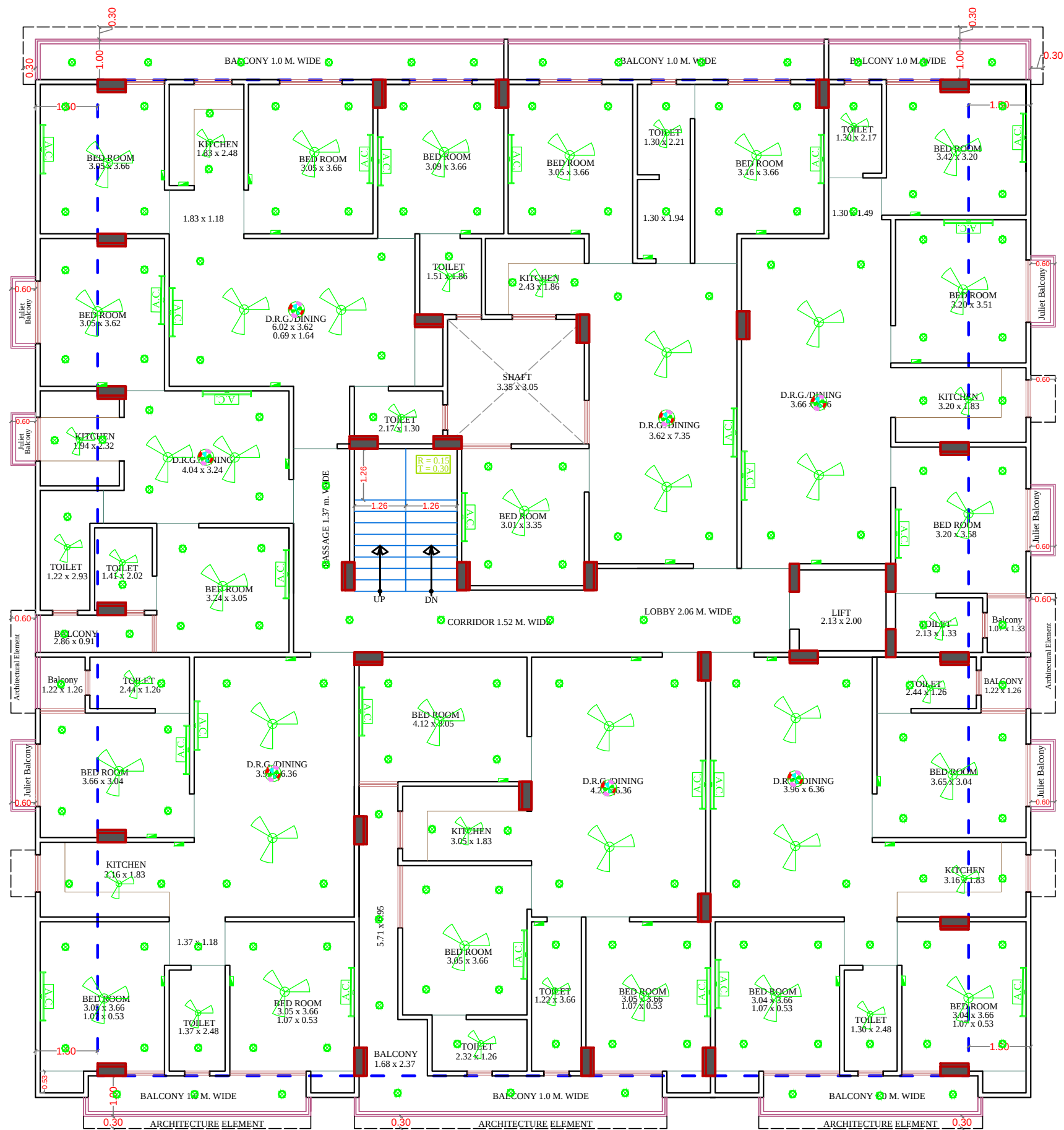
GROUND, 1st TO 5th FLOOR PLAN
