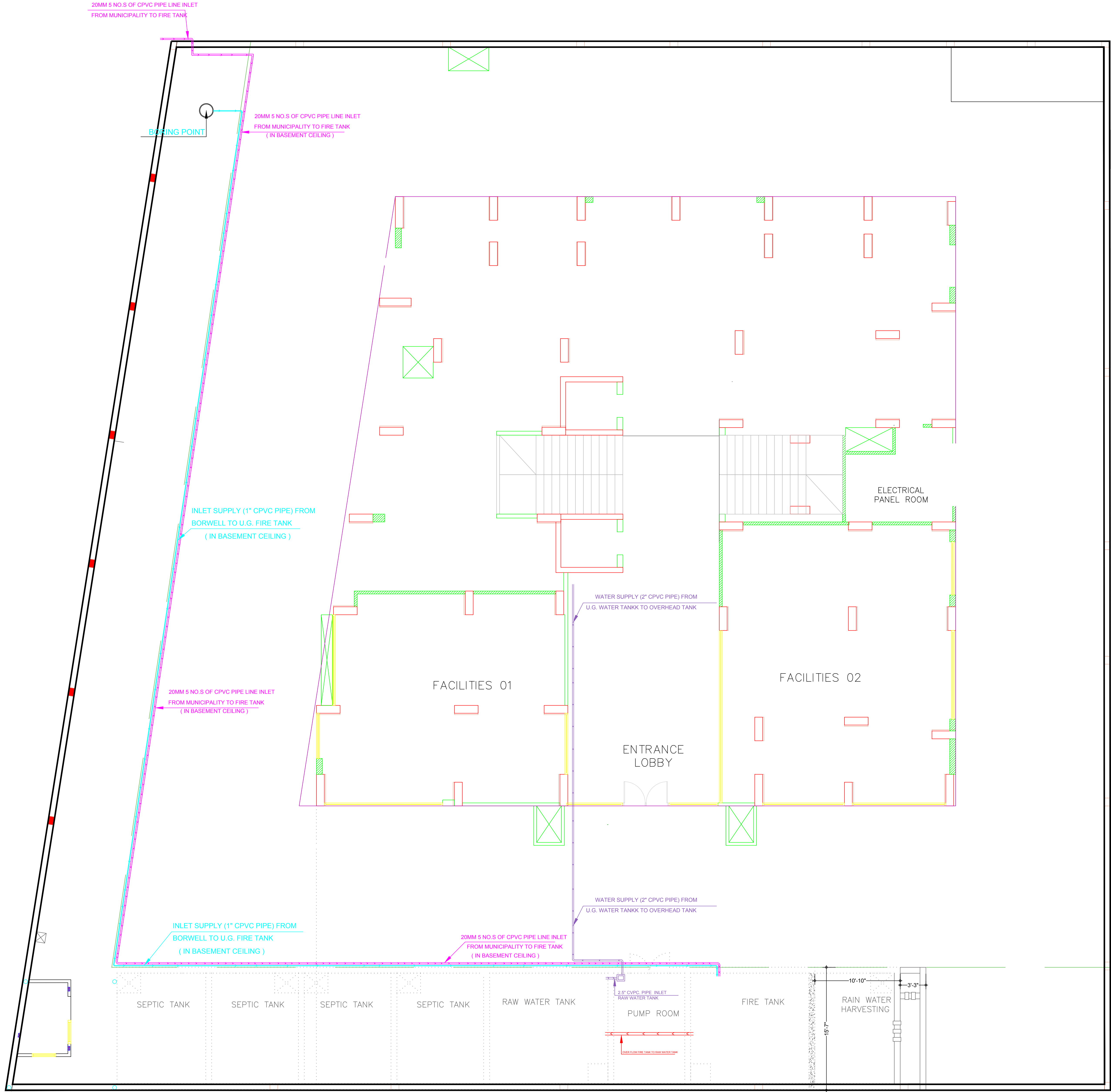
STILT FLOOR PLAN (WATER SUPPLY )
