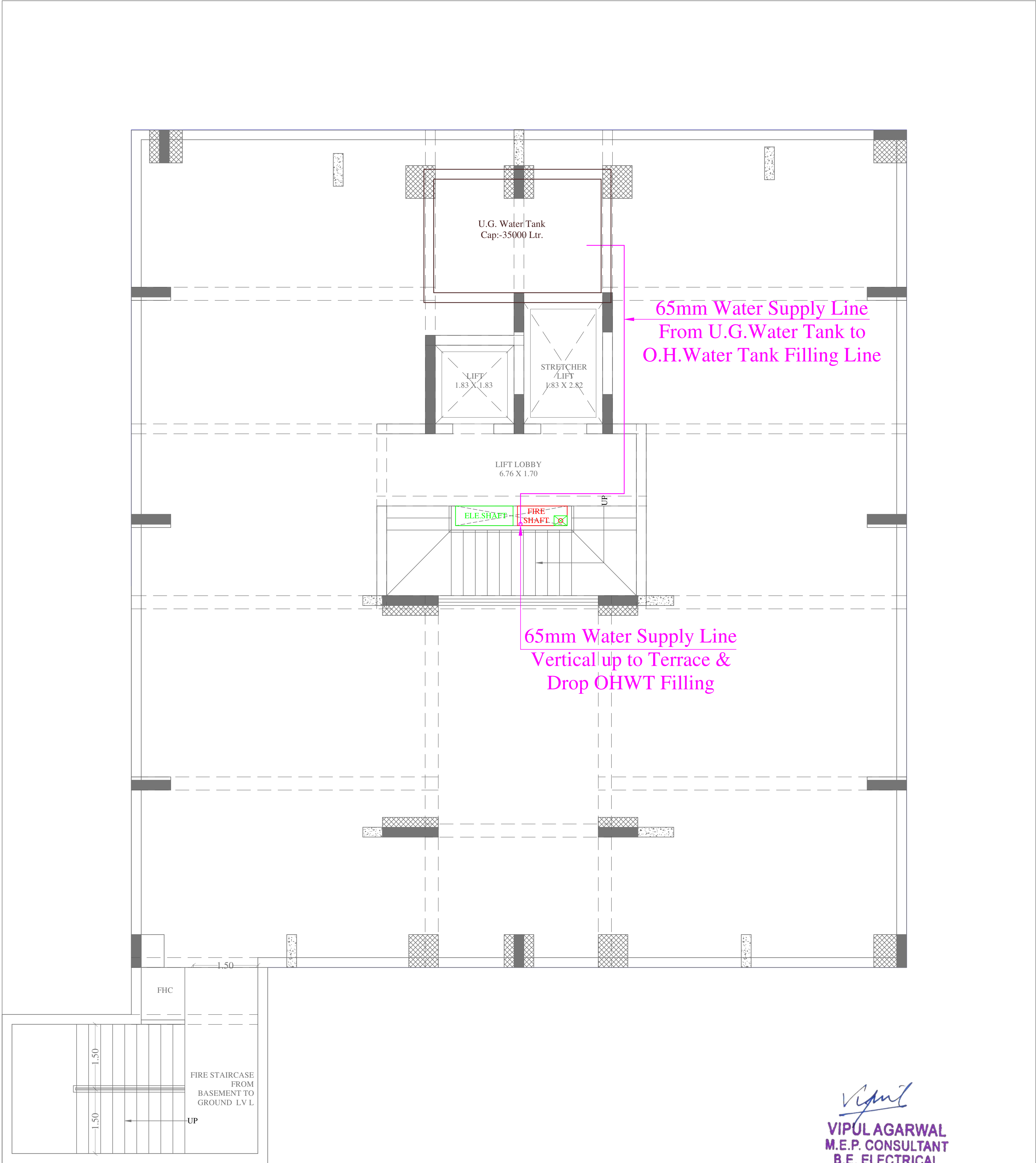
BASEMENT FLOOR
