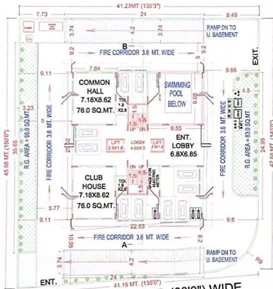
STILT FLOOR PLAN MEP SERVICES LAYOUT
