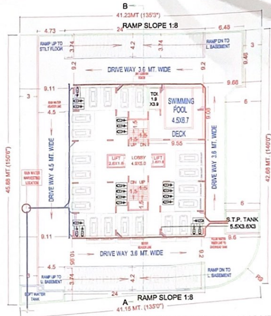
UPPER BASEMENT MEP SERVICES LAYOUT
