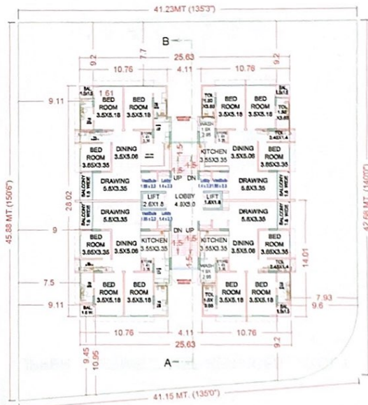
TYPICAL FLOOR WATER SUPPLY LAYOUT
