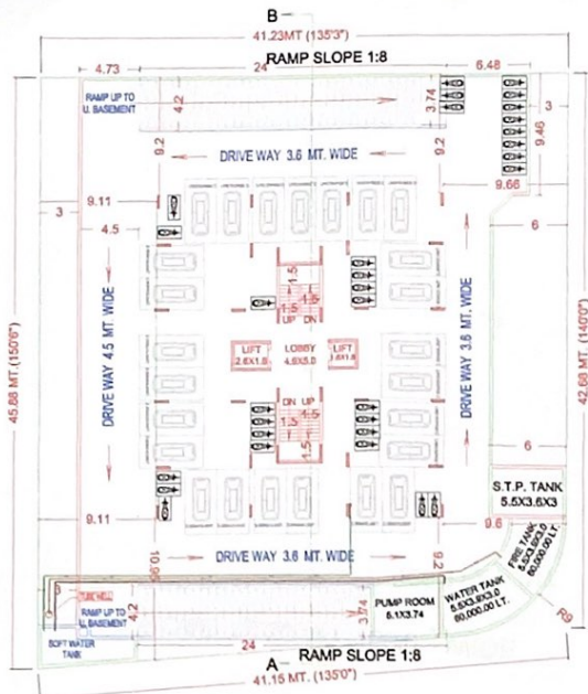
LOWER BASEMENT MEP SERVICES LAYOUT
