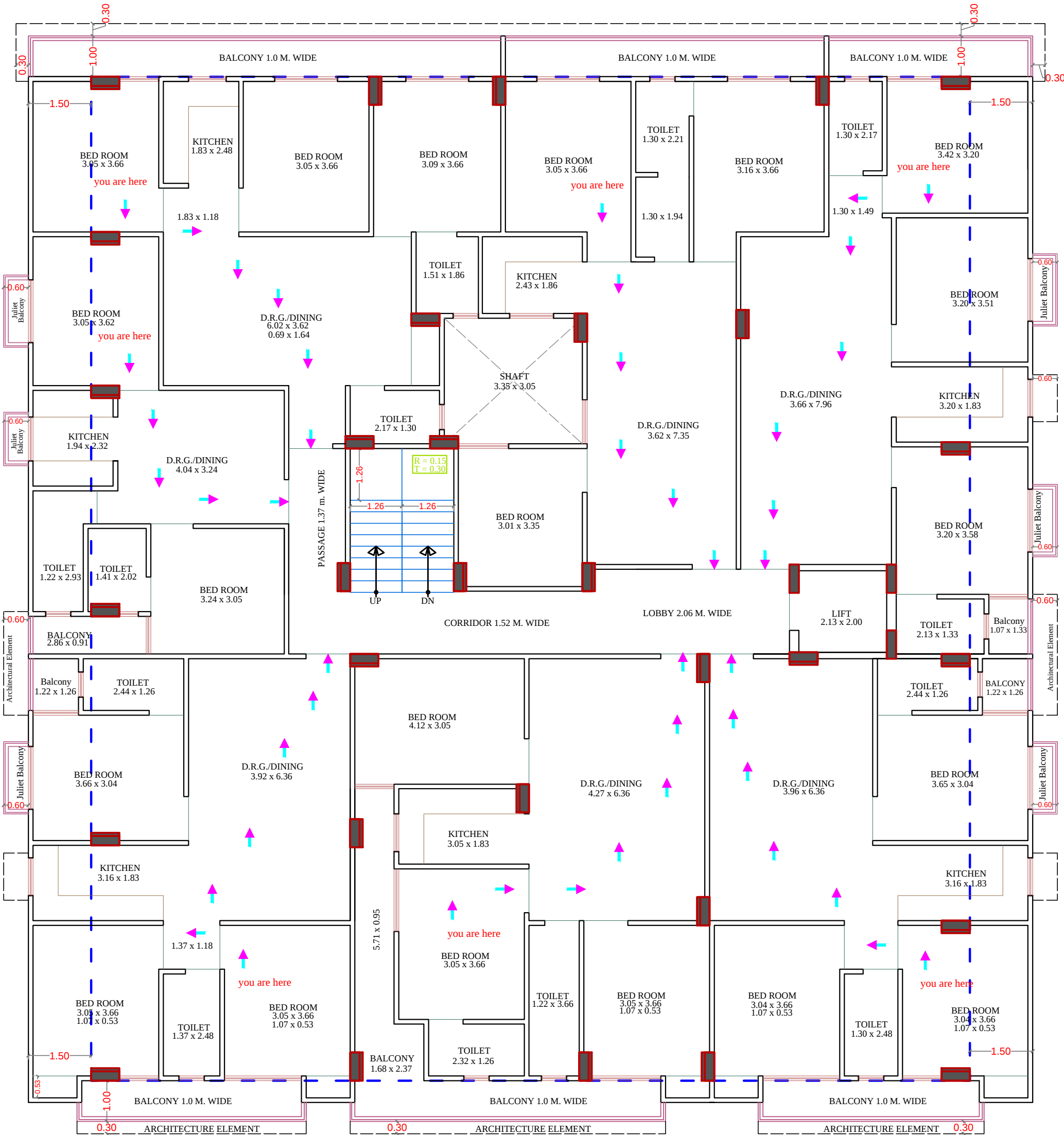
GROUND, 1st TO 5th FLOOR PLAN
