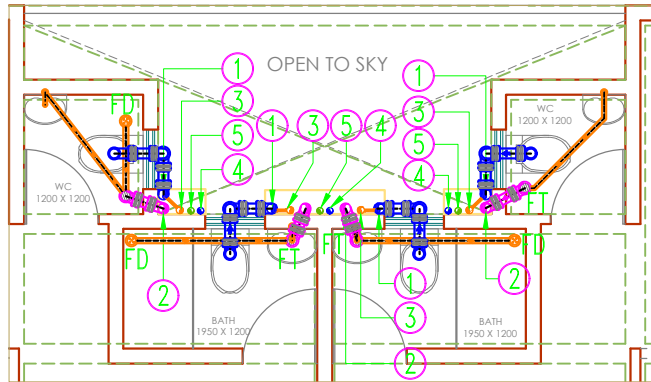
TYPICAL FLOOR TOILET DETAIL-02 DRAINAGE LAYOUT
