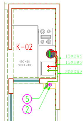
TYPICAL FLOOR KITCHEN DETAIL-02 WATER SUPPLY LAYOUT
