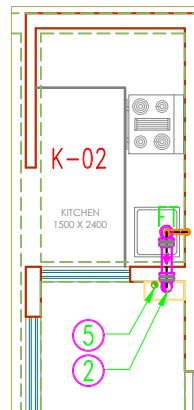
TYPICAL FLOOR KITCHEN DETAIL-02 DRAINAGE LAYOUT
