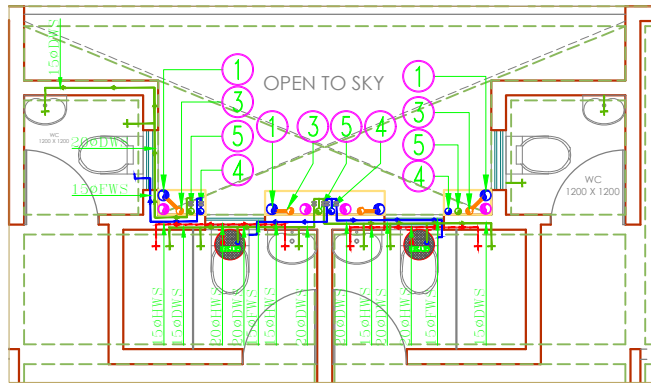
TYPICAL FLOOR TOILET DETAIL-02 WATER SUPPLY LAYOUT
