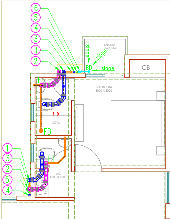
TYPICAL FLOOR TOILET DETAIL-01 DRAINAGE LAYOUT
