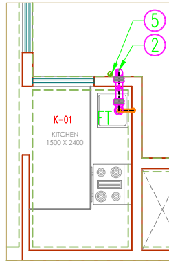
TYPICAL FLOOR KITCHEN DETAIL-01 DRAINAGE LAYOUT
