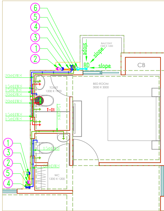
TYPICAL FLOOR TOILET DETAIL-01 WATER SUPPLY LAYOUT
