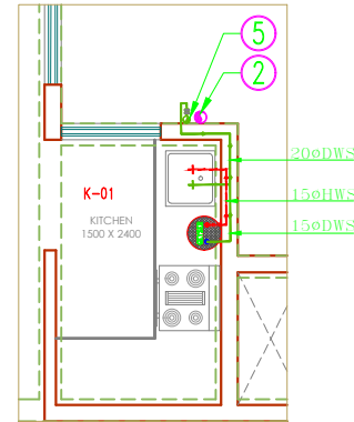
TYPICAL FLOOR KITCHEN DETAIL-01 WATER SUPPLY LAYOUT
