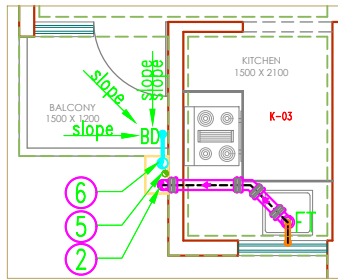
TYPICAL FLOOR KITCHEN DETAIL-03 DRAINAGE LAYOUT
