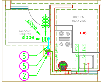
TYPICAL FLOOR KITCHEN DETAIL-03 WATER SUPPLY LAYOUT
