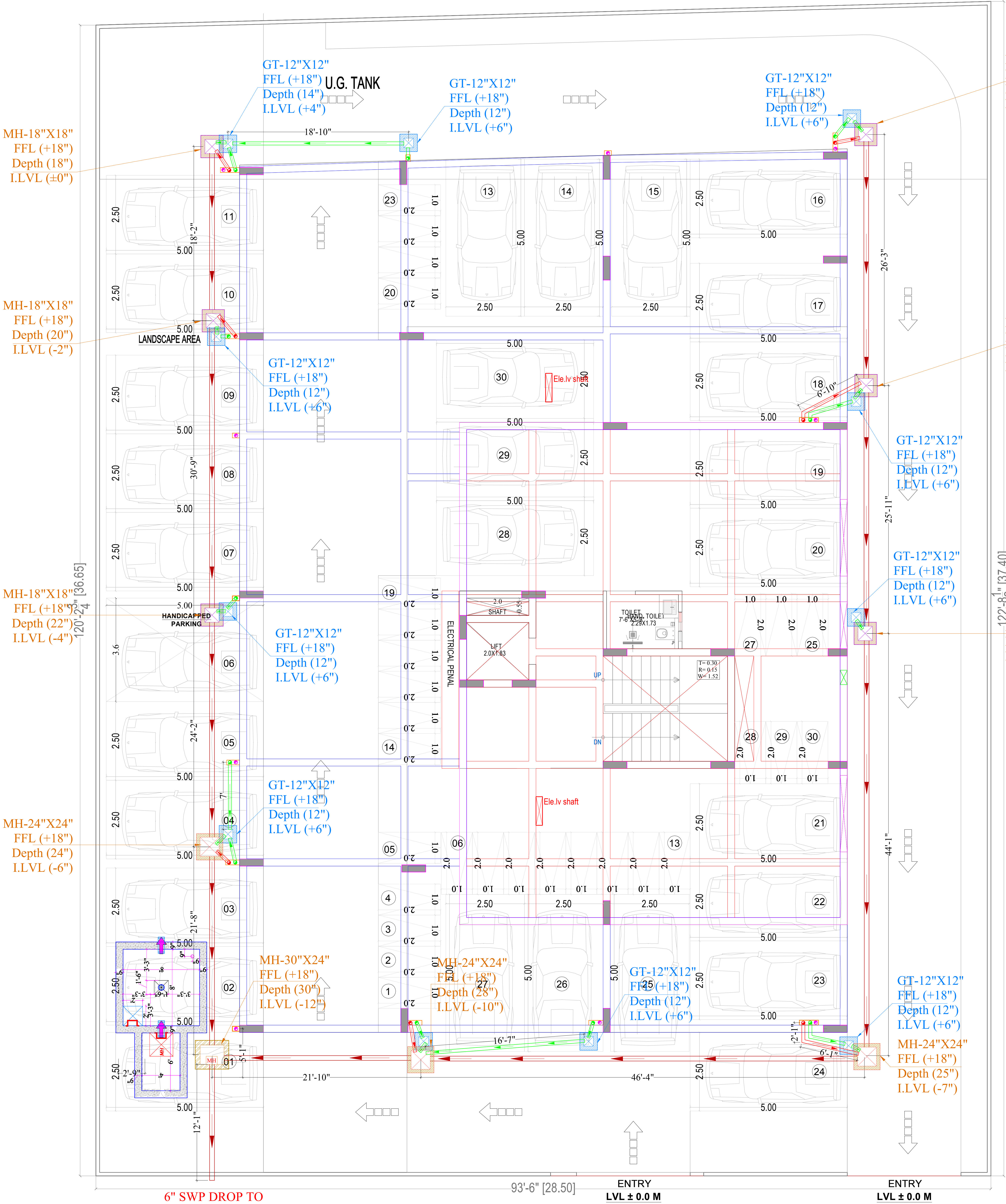
STILT FLOOR & PARKING PLAN
