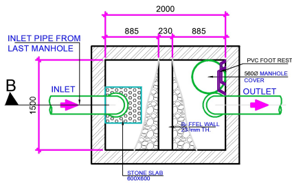
PLAN OF DESILTING CHAMBER & RWH PIT
