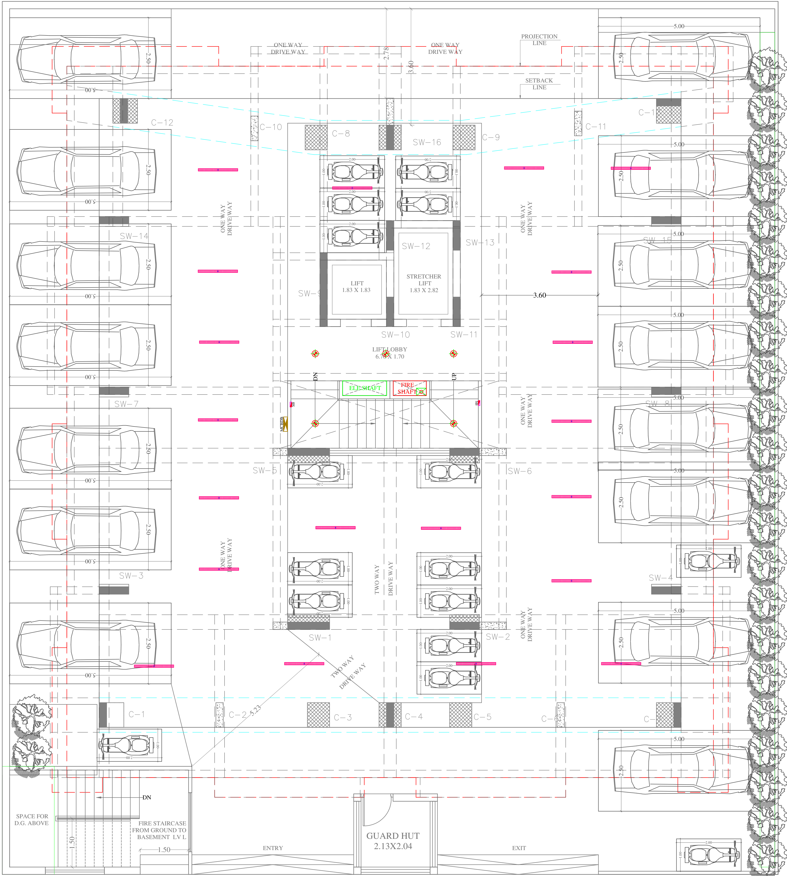
STILT FLOOR PLAN
