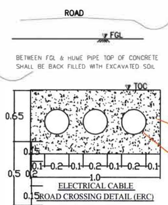
SECTION T1-T1
