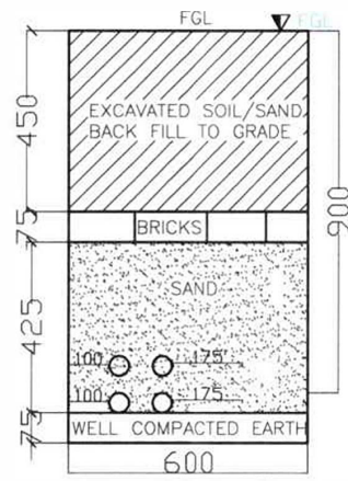
SECTION- T2-T2
