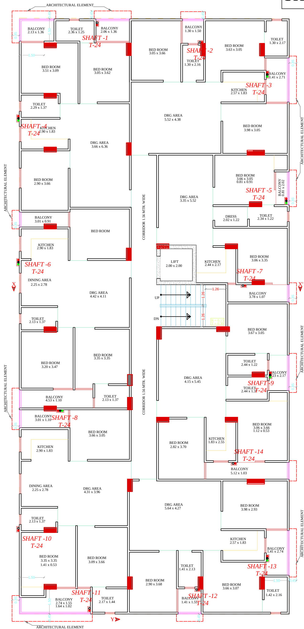
GROUND, 1st TO 5th FLOOR PLAN
