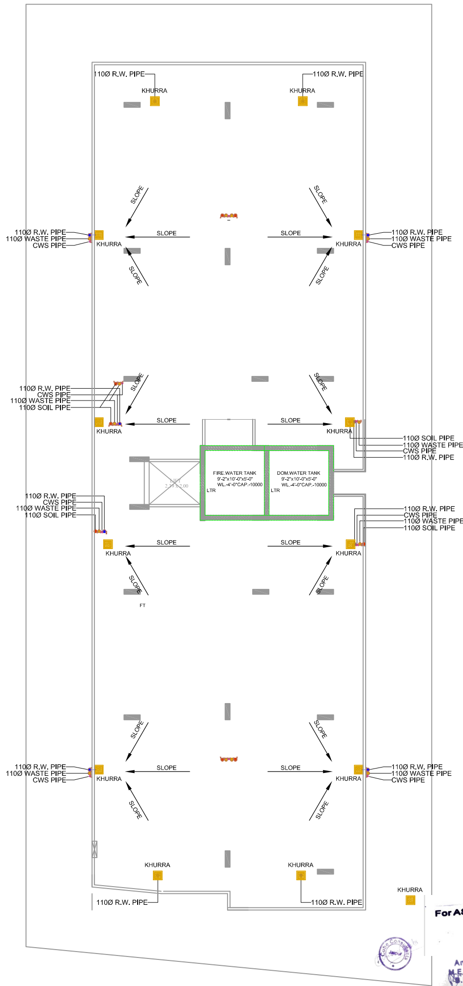
PROPOSED TERRACE FLOOR DRAINAGE LAYOUT
