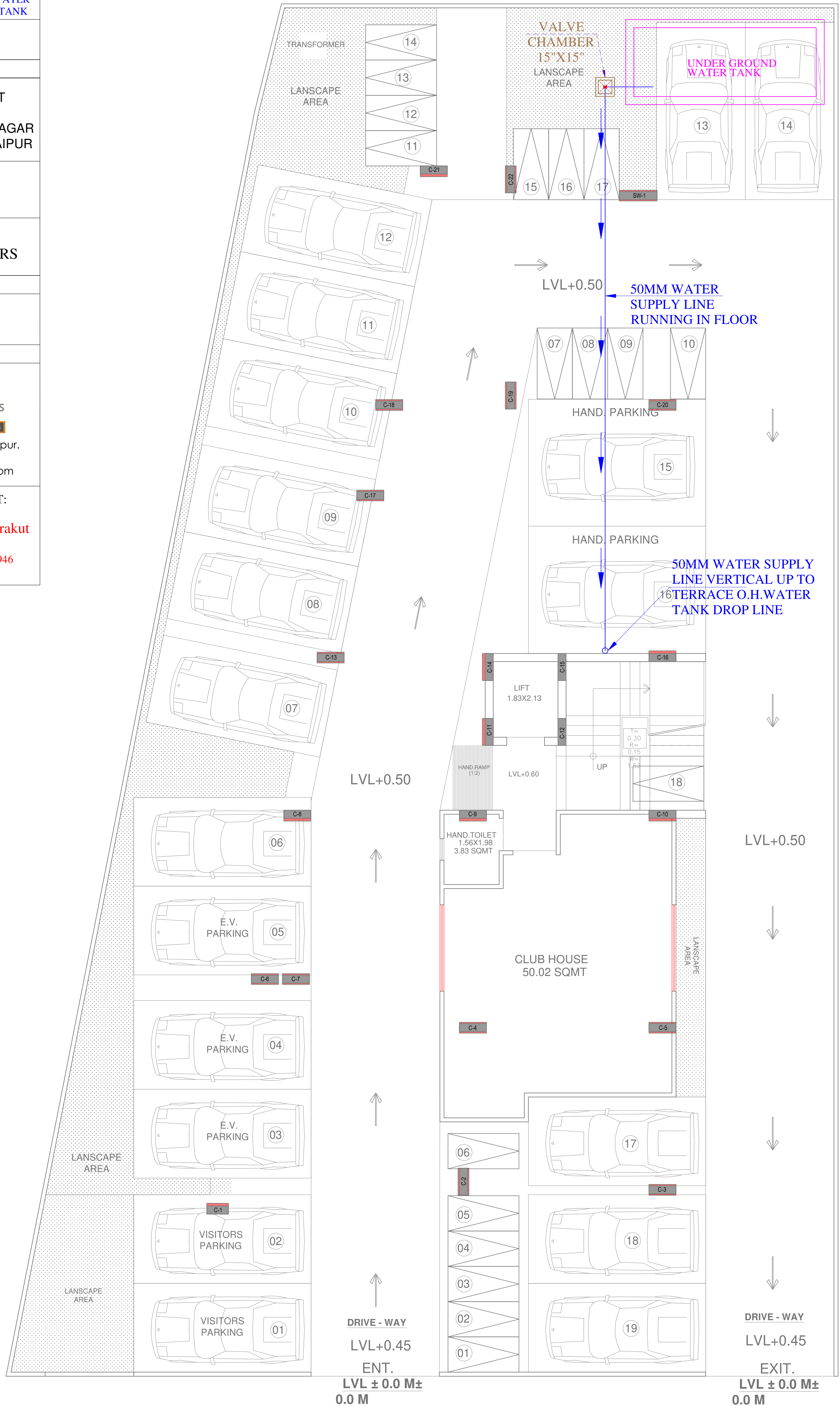
STILT FLOOR PLAN
