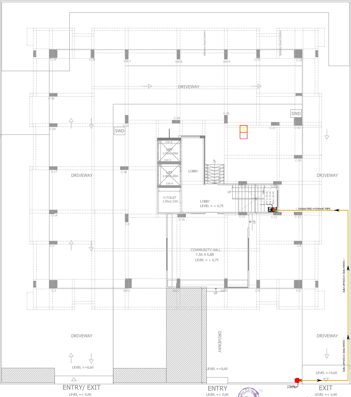
PROPOSED STILT FLOOR FIRE FIGHTING LAYOUT
