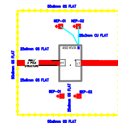
Detail-1,2,3 Switch Yard Layout Plan
