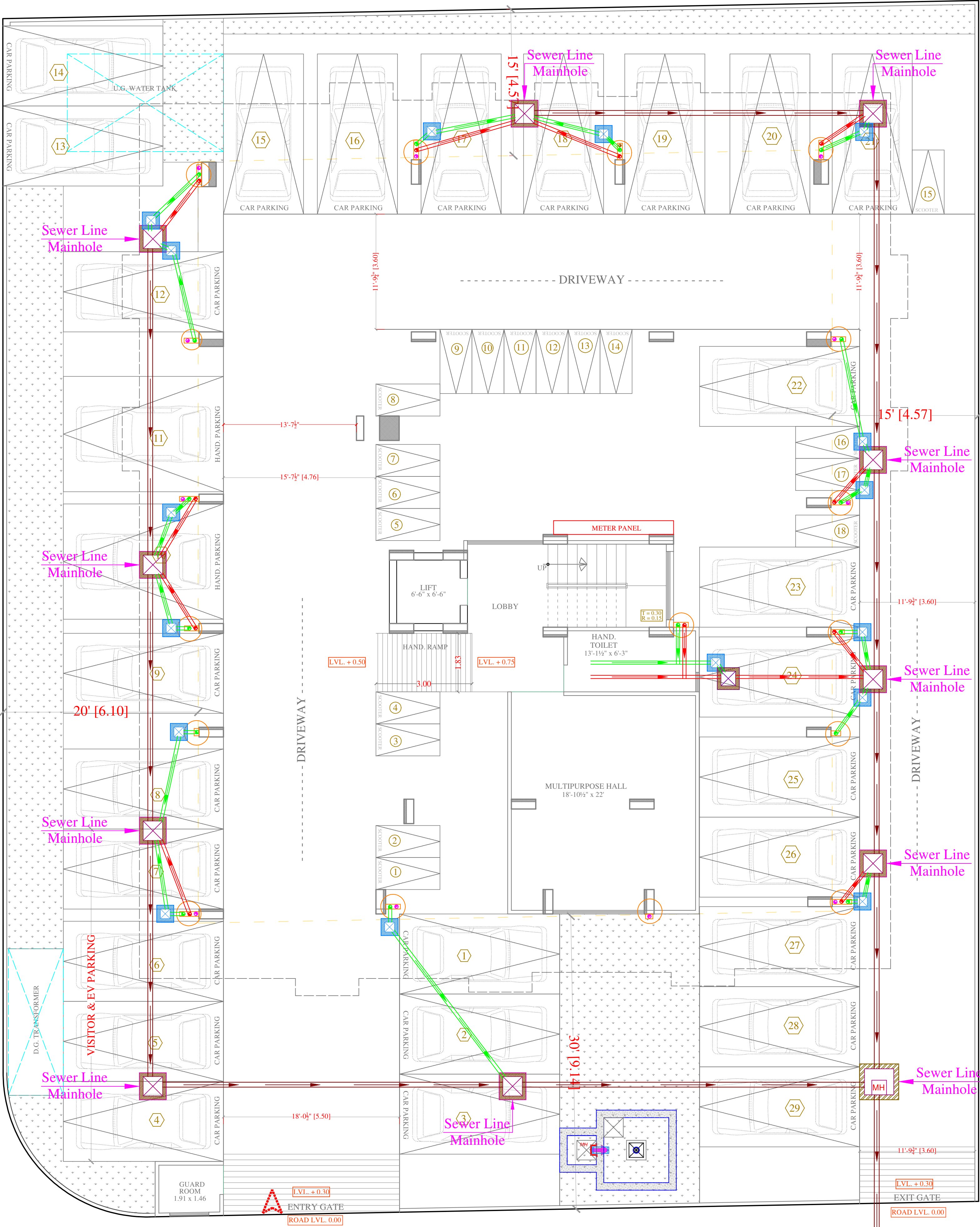
STILT PLAN
