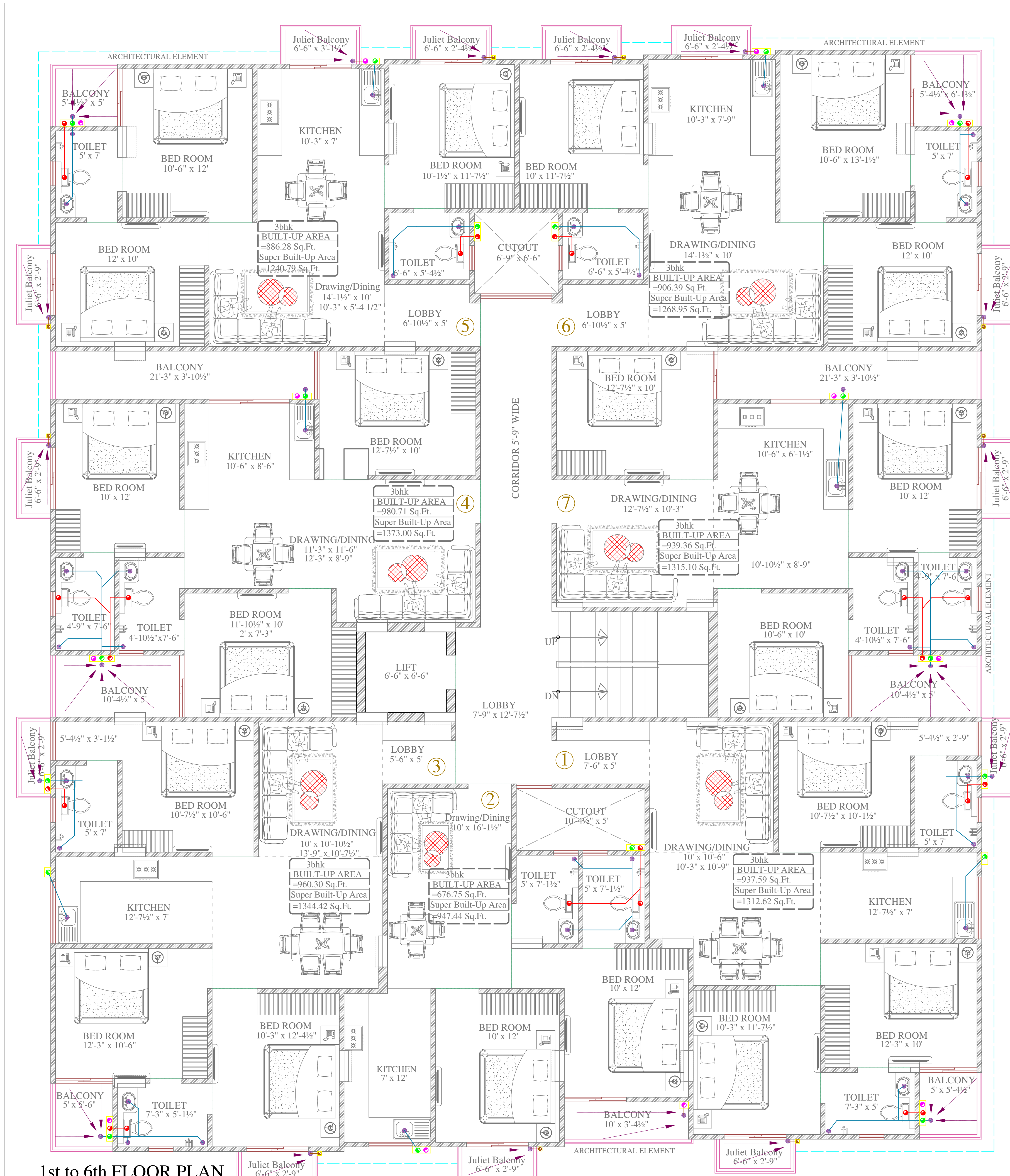
1st to 6th FLOOR PLAN
