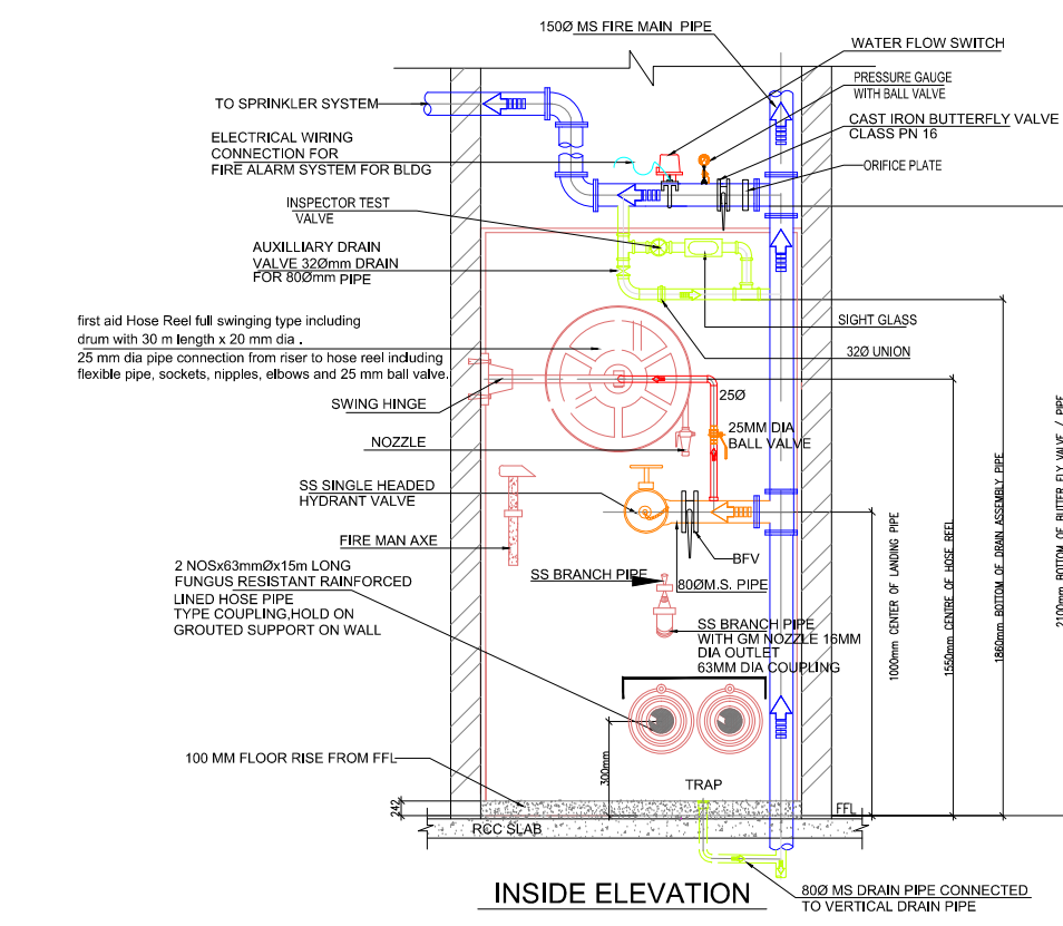
TYPICAL FIRE HOSE CABINET DETAIL
