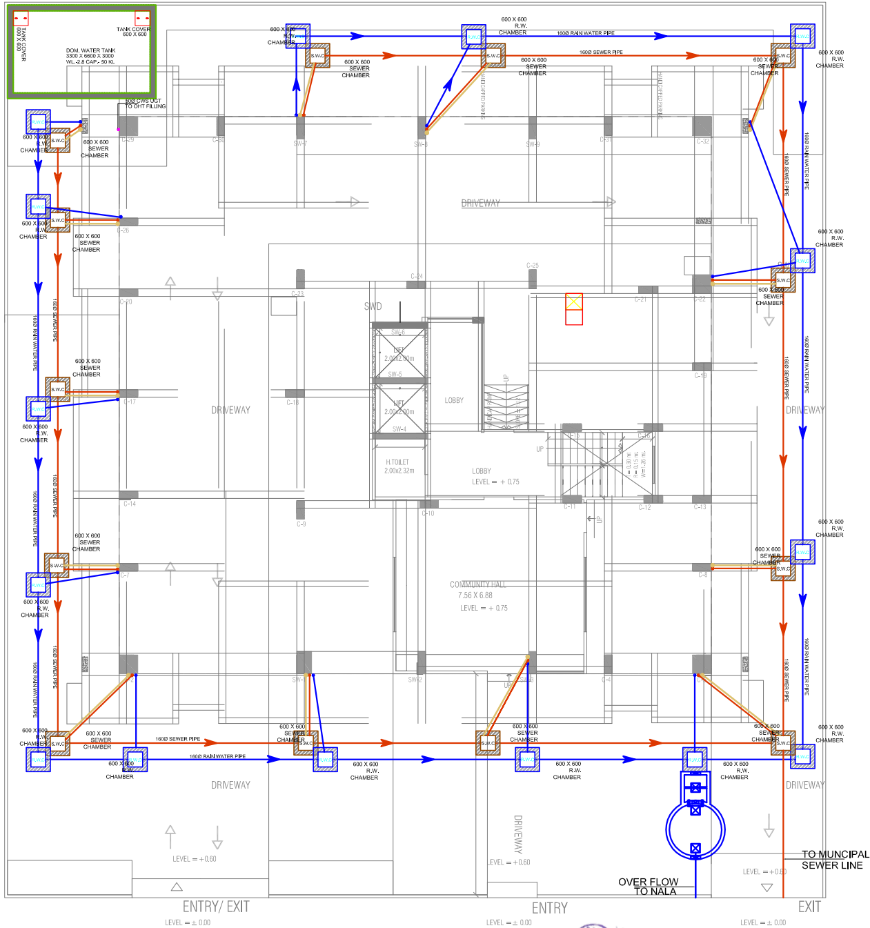
STILT FLOOR RAIN WATER HARVESTING COMMON WATER PIPE ROUTE PLAN
