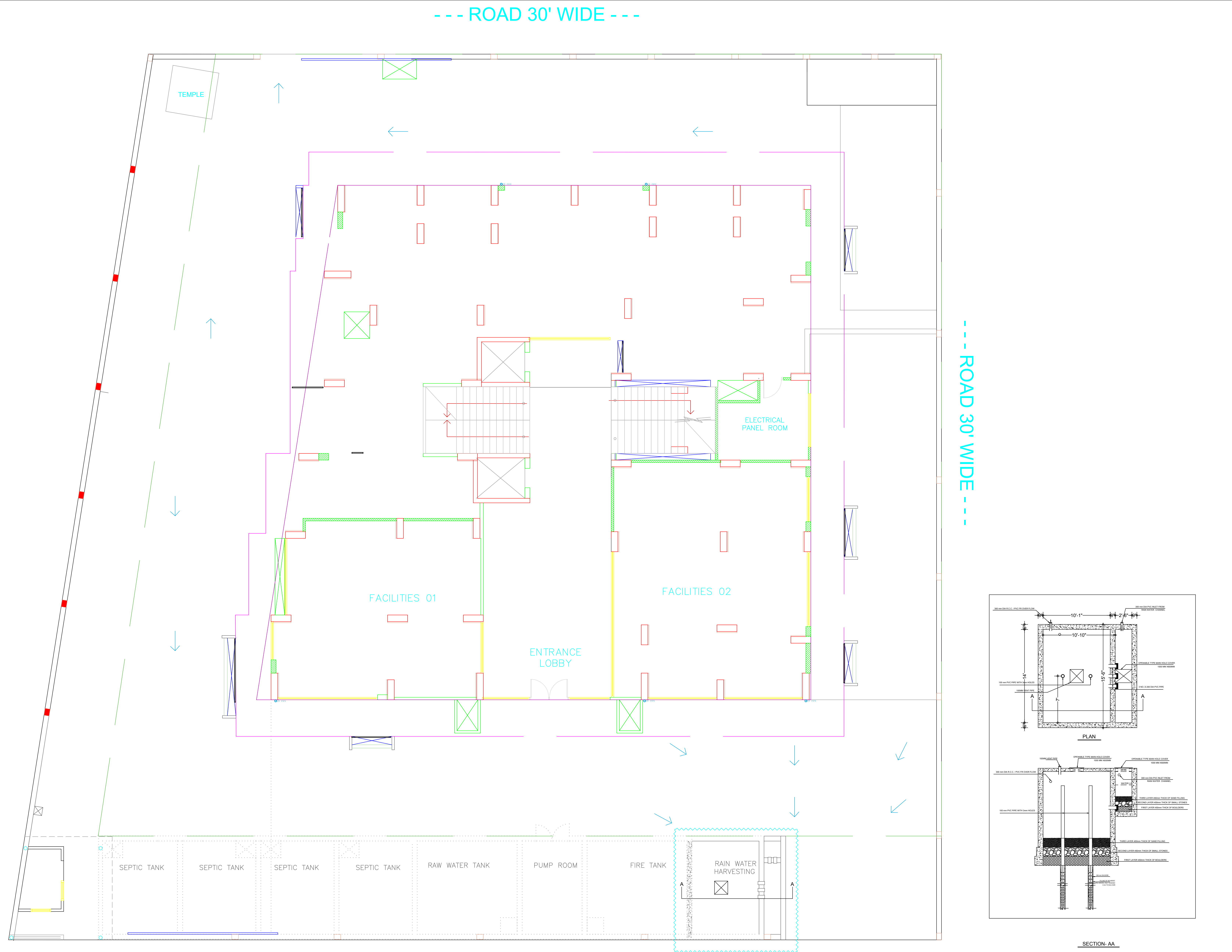
STILT FLOOR PLAN (RAIN WATER HARVESTING )
