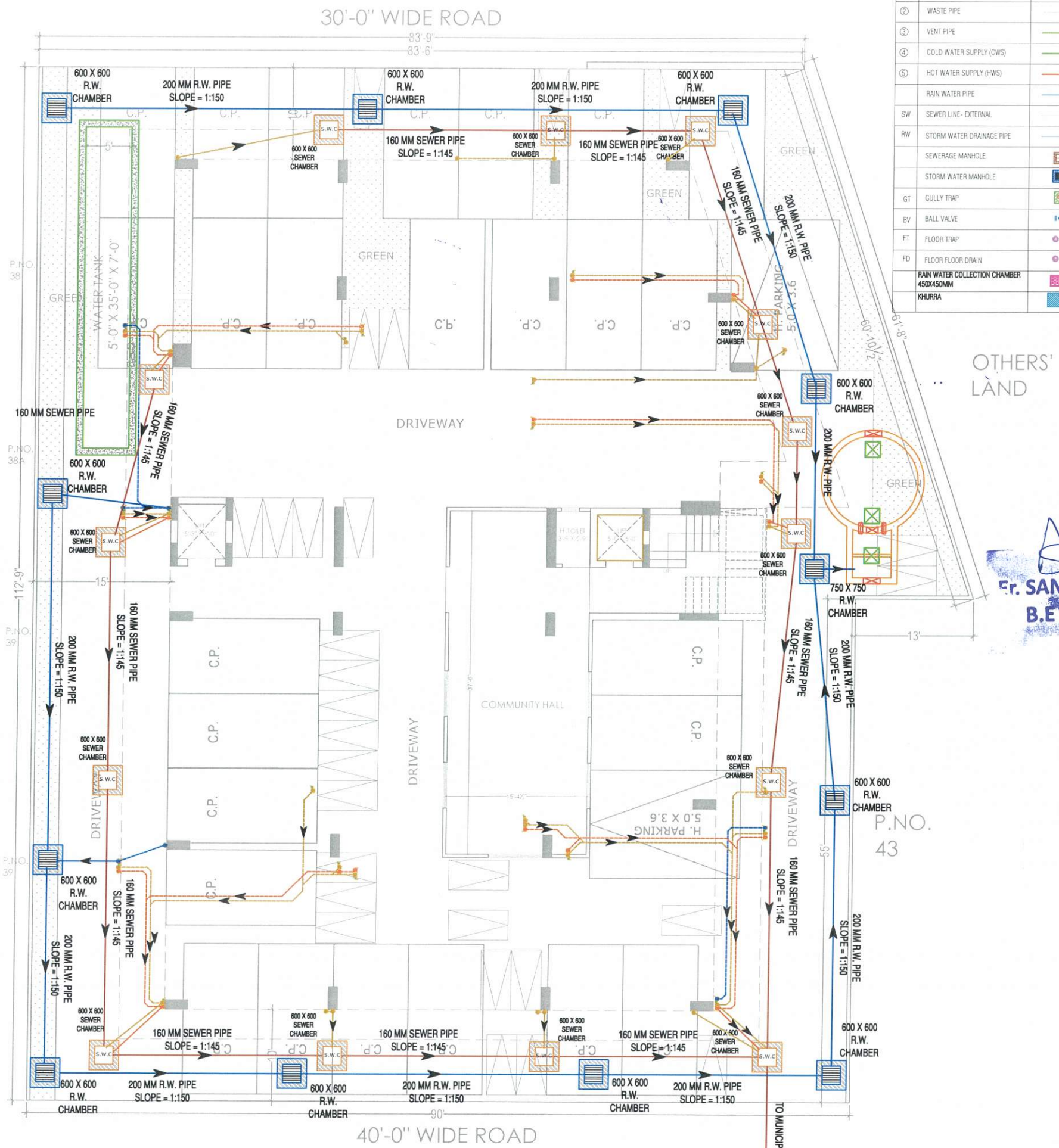
STILT FLOOR DRAINAGE LAYOUT PLAN
