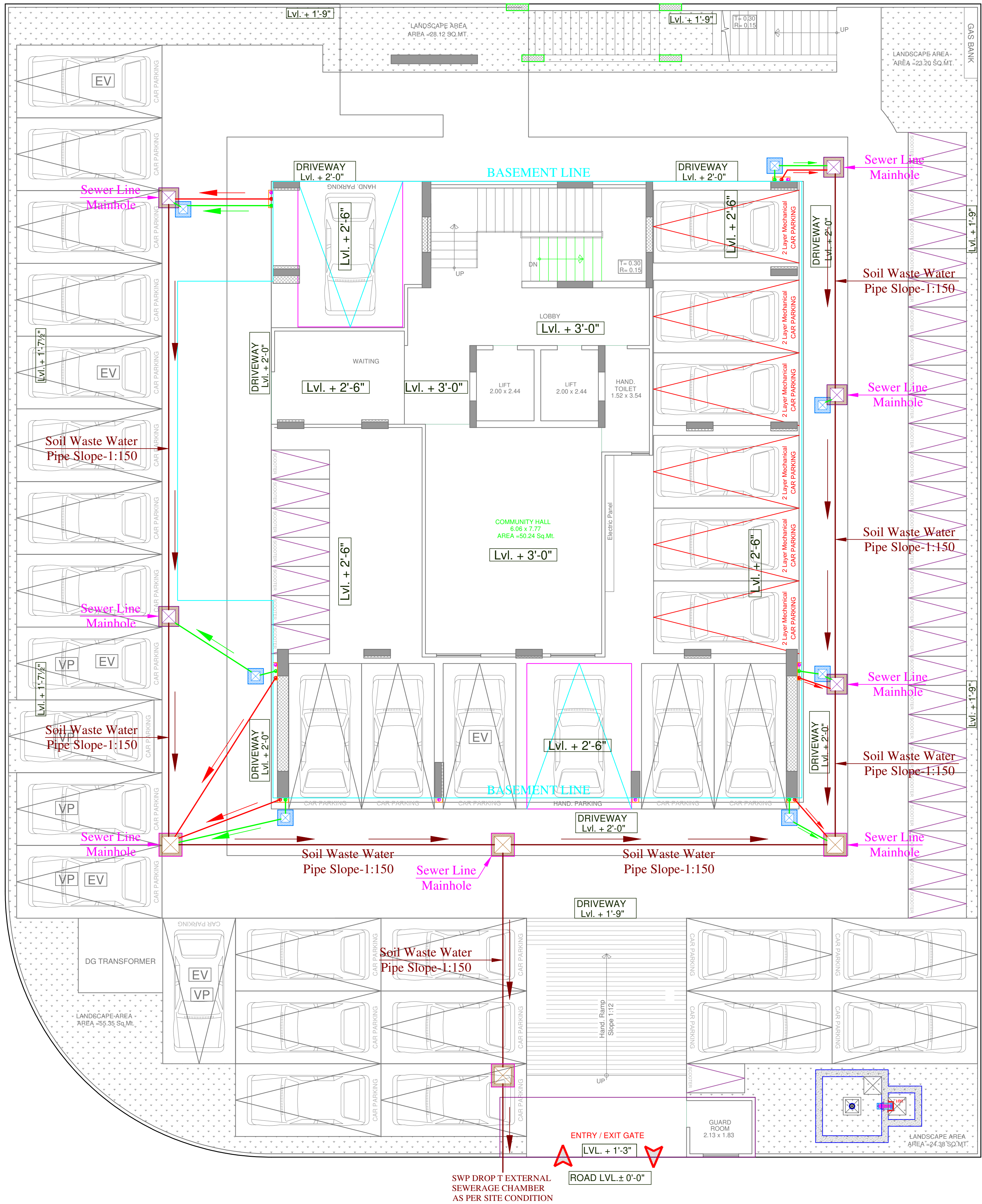
STILT PLAN
