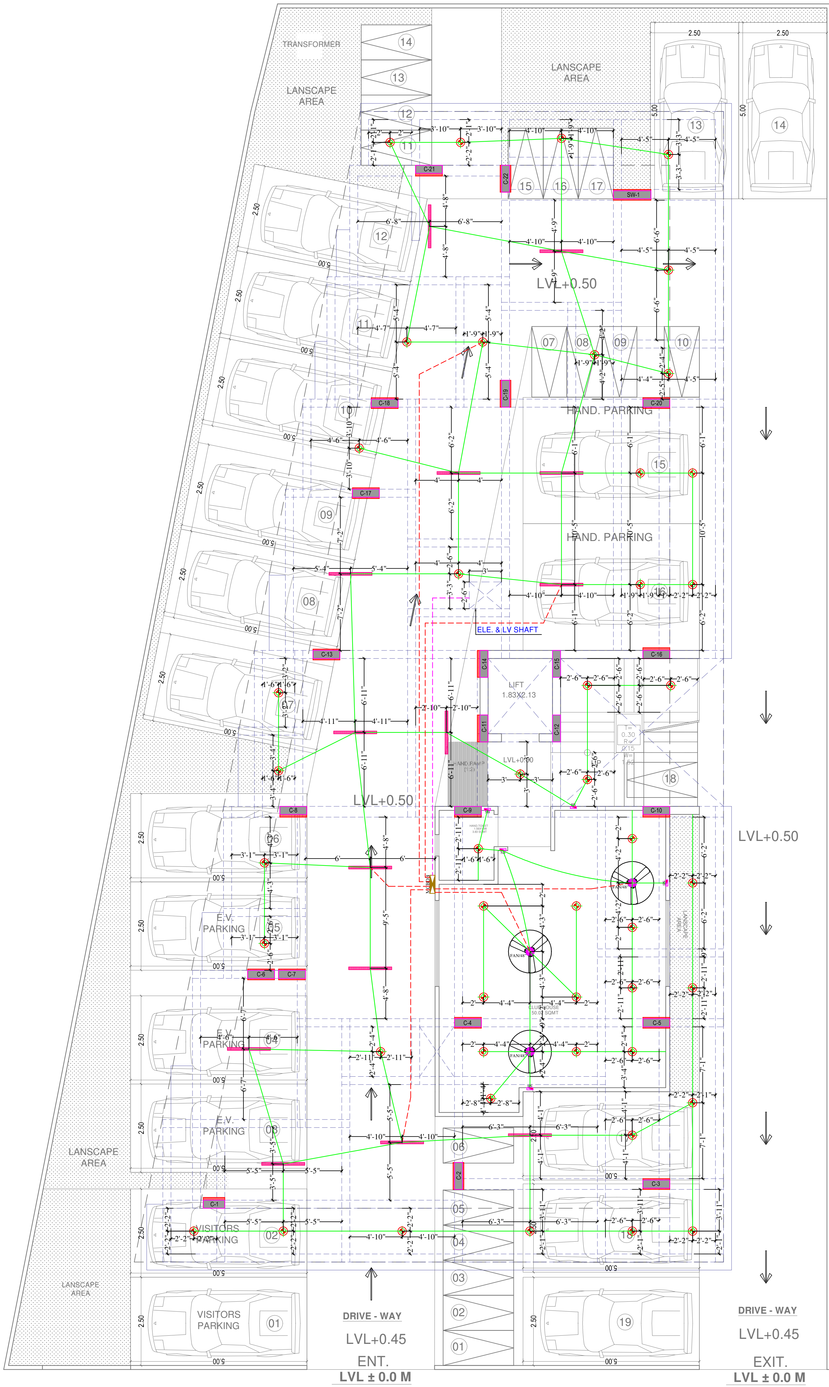
STILT FLOOR PLAN
