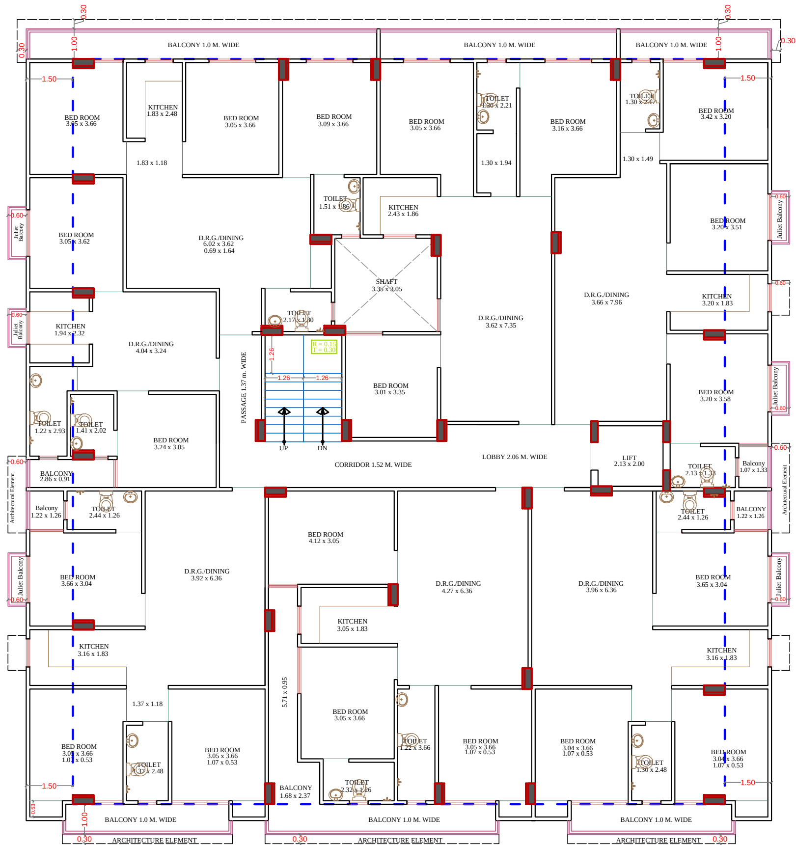
GROUND, 1st TO 5th FLOOR PLAN
