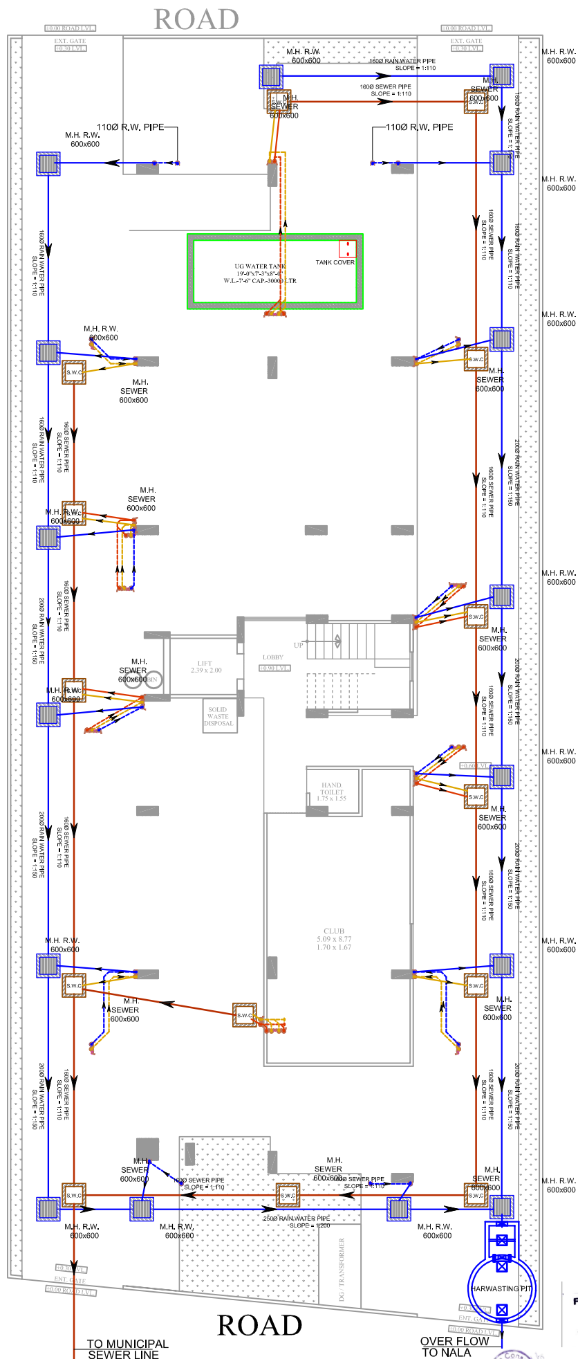
PROPOSED STILT FLOOR PIPE ROUTE & RAIN WATER HARWASTING PIT LAYOUT
