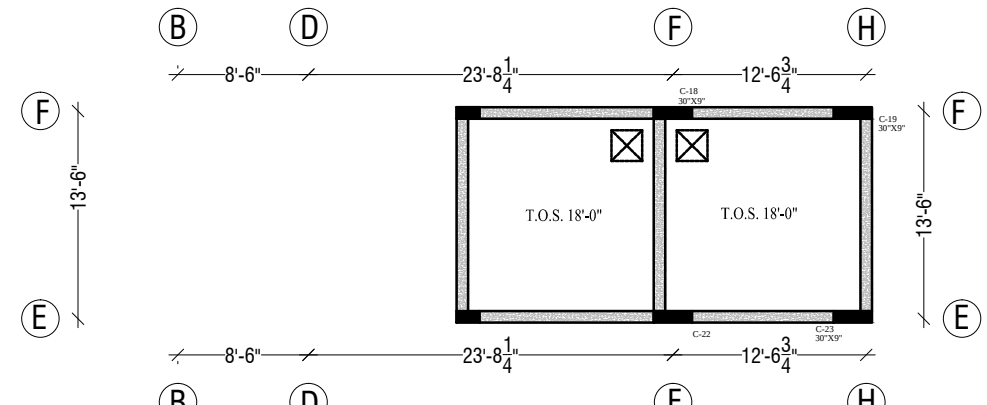
WATER TANK TOP LEVEL SHUTTERING PLAN
