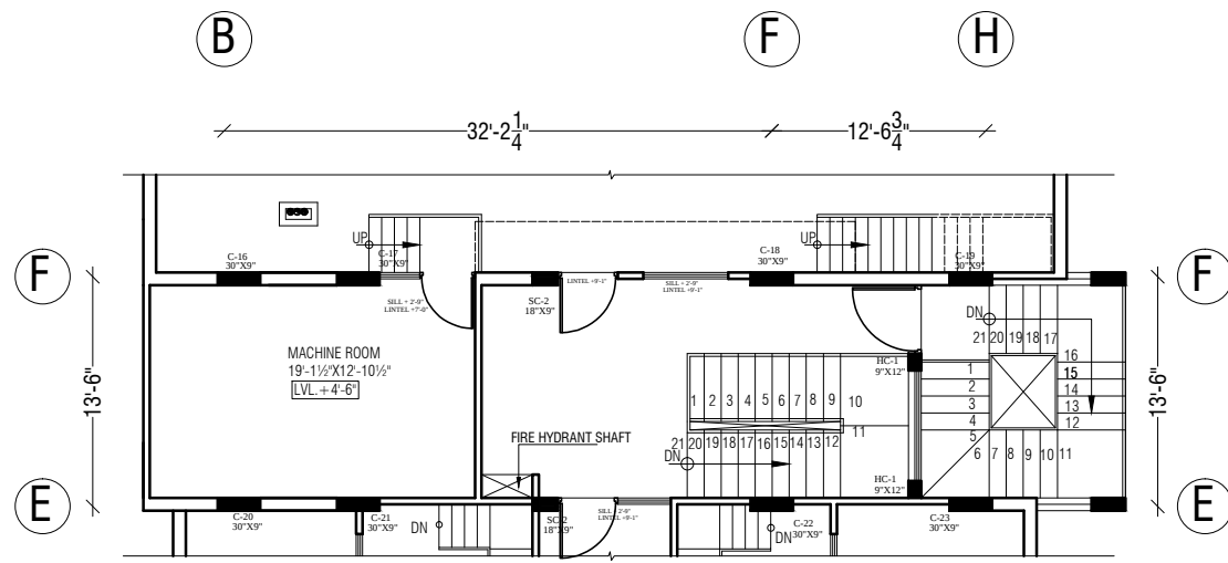
TERRACE FLOOR PART PLAN
