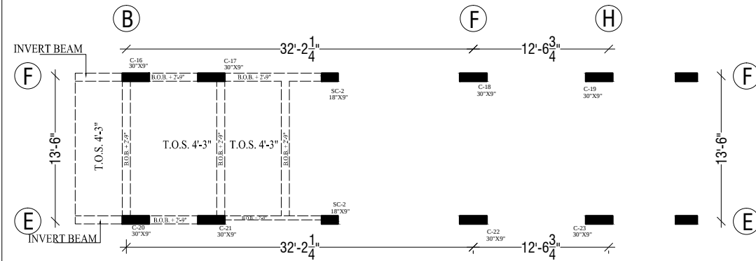
MACHINE ROOM FLOOR LEVEL SHUTTERING PLAN
