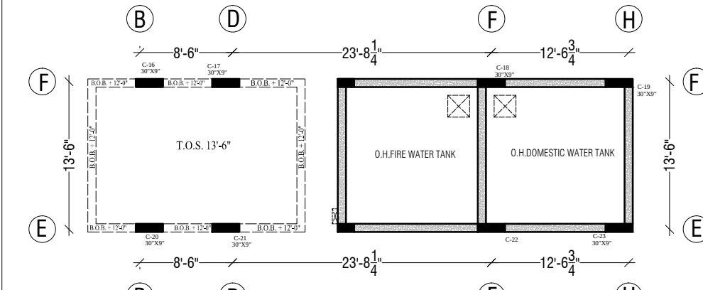
MACHINE ROOM ROOF SHUTTERING PLAN
