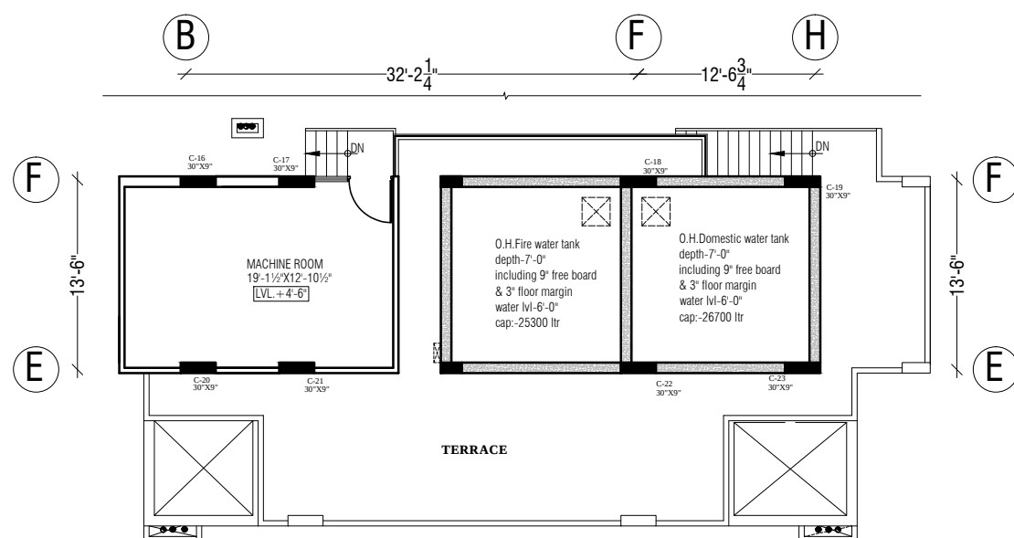
MUMTY ROOF FLOOR PLAN
