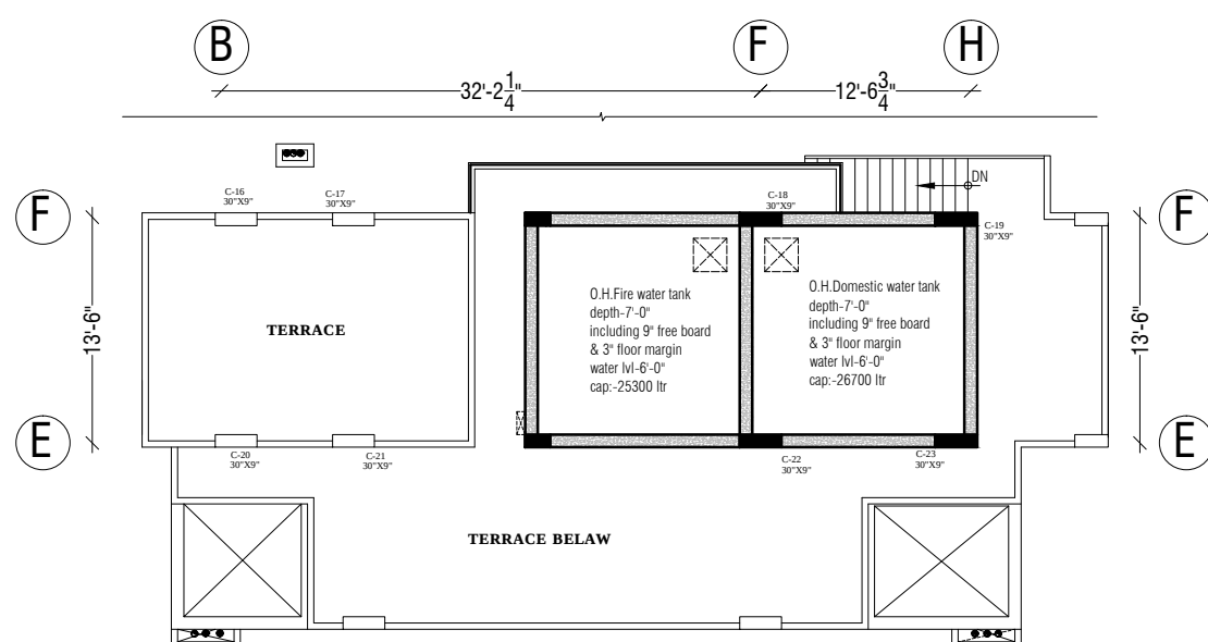
MACHINE ROOM ROOF FLOOR PLAN
