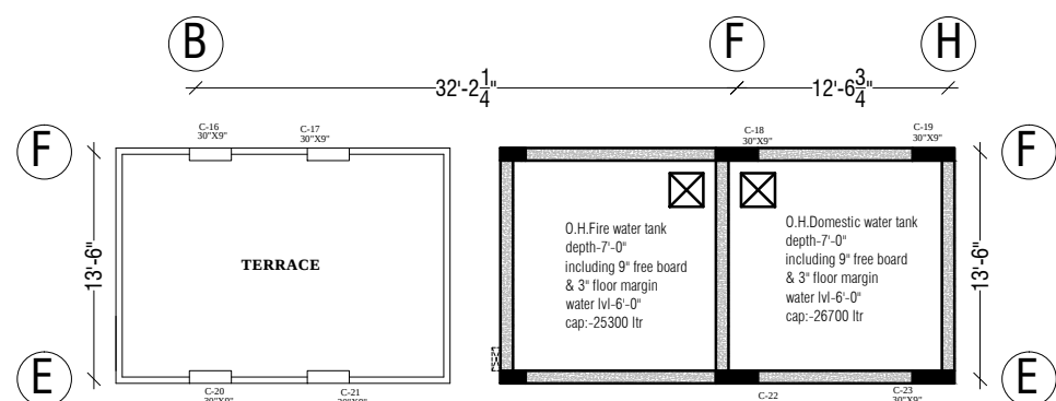
WATER TANK TOP PLAN
