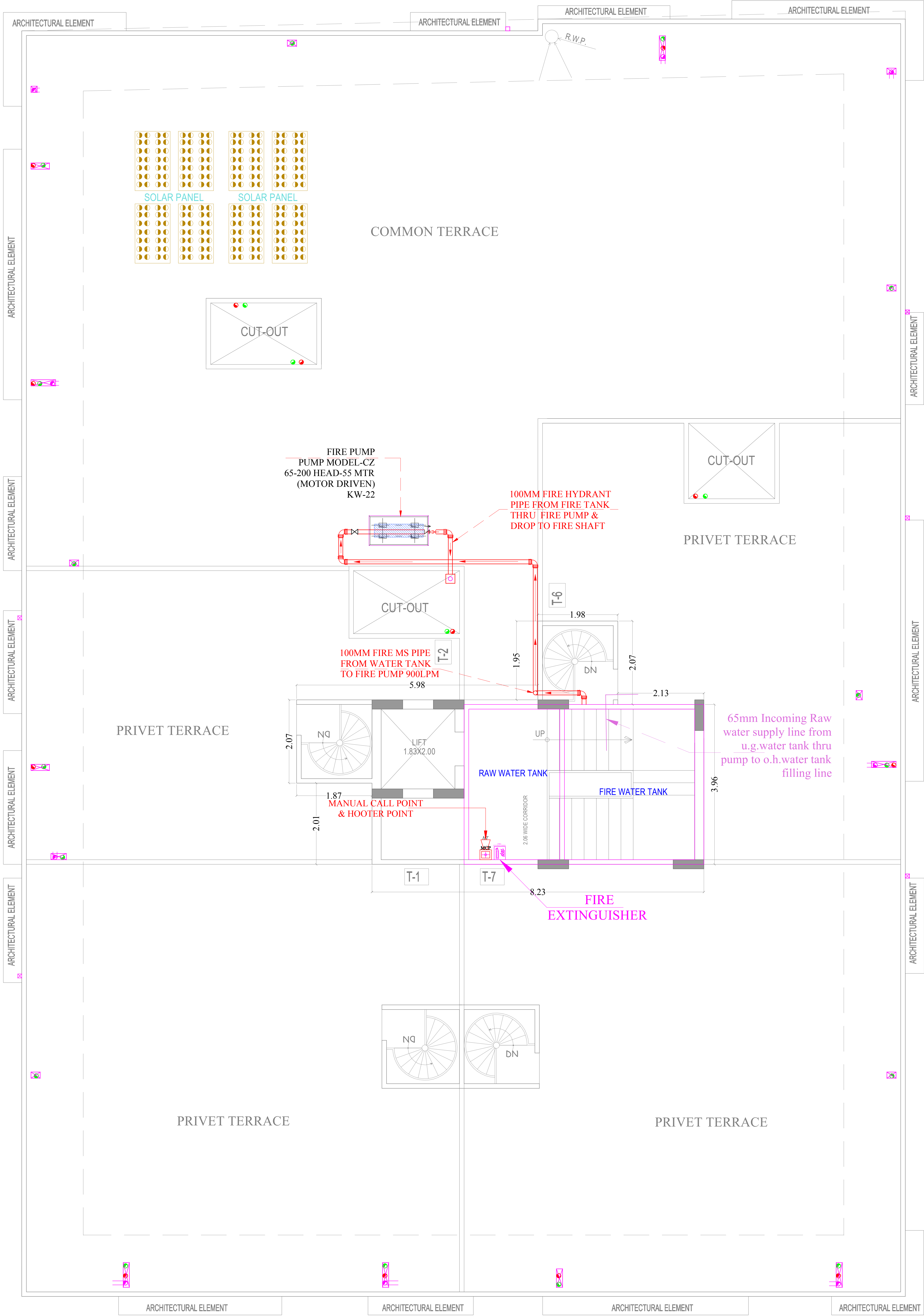
TERRACE FLOOR PLAN
