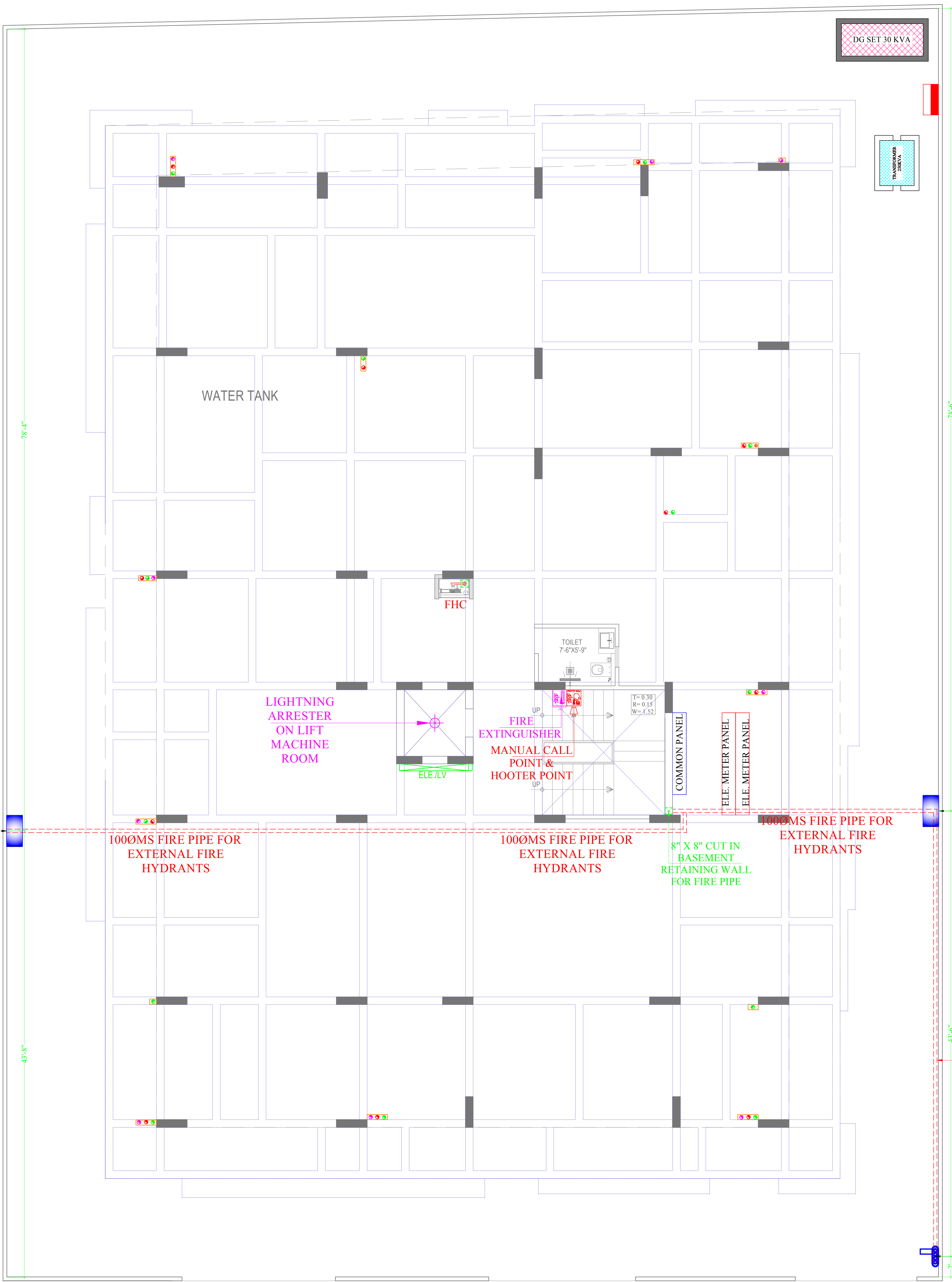
STILT FLOOR PLAN
