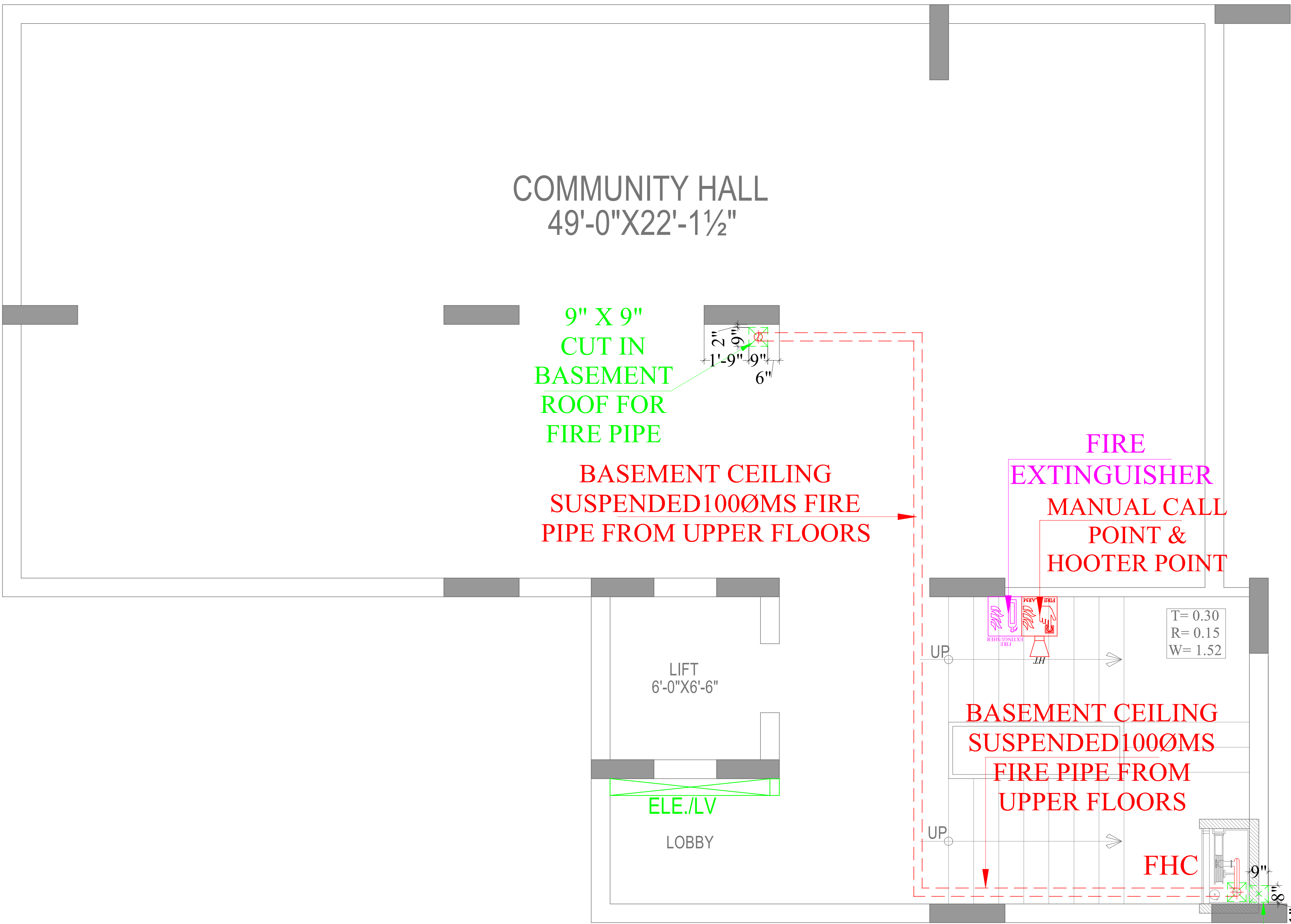
BASEMENT FLOOR PLAN
