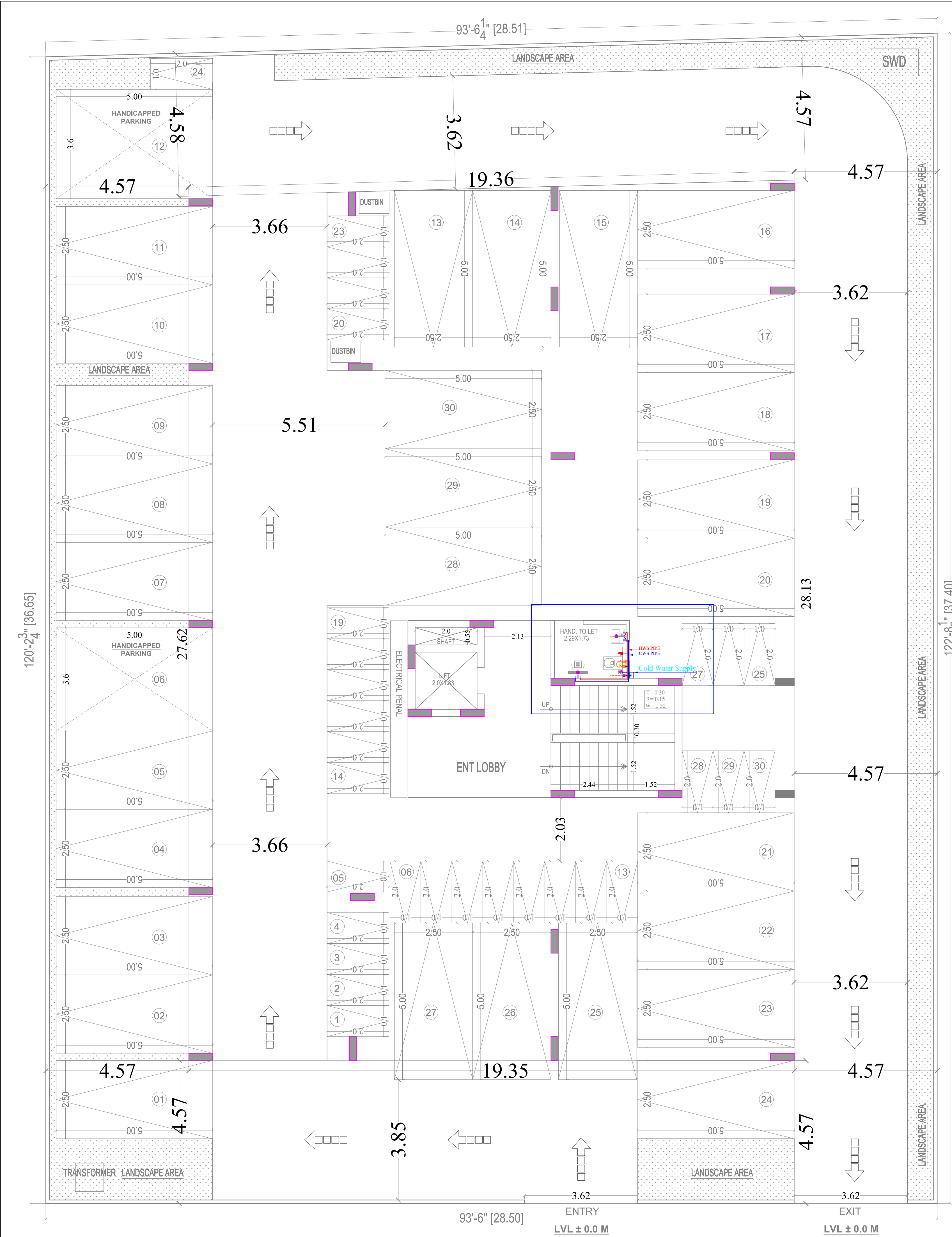
STILT & PARKING FLOOR PLAN
