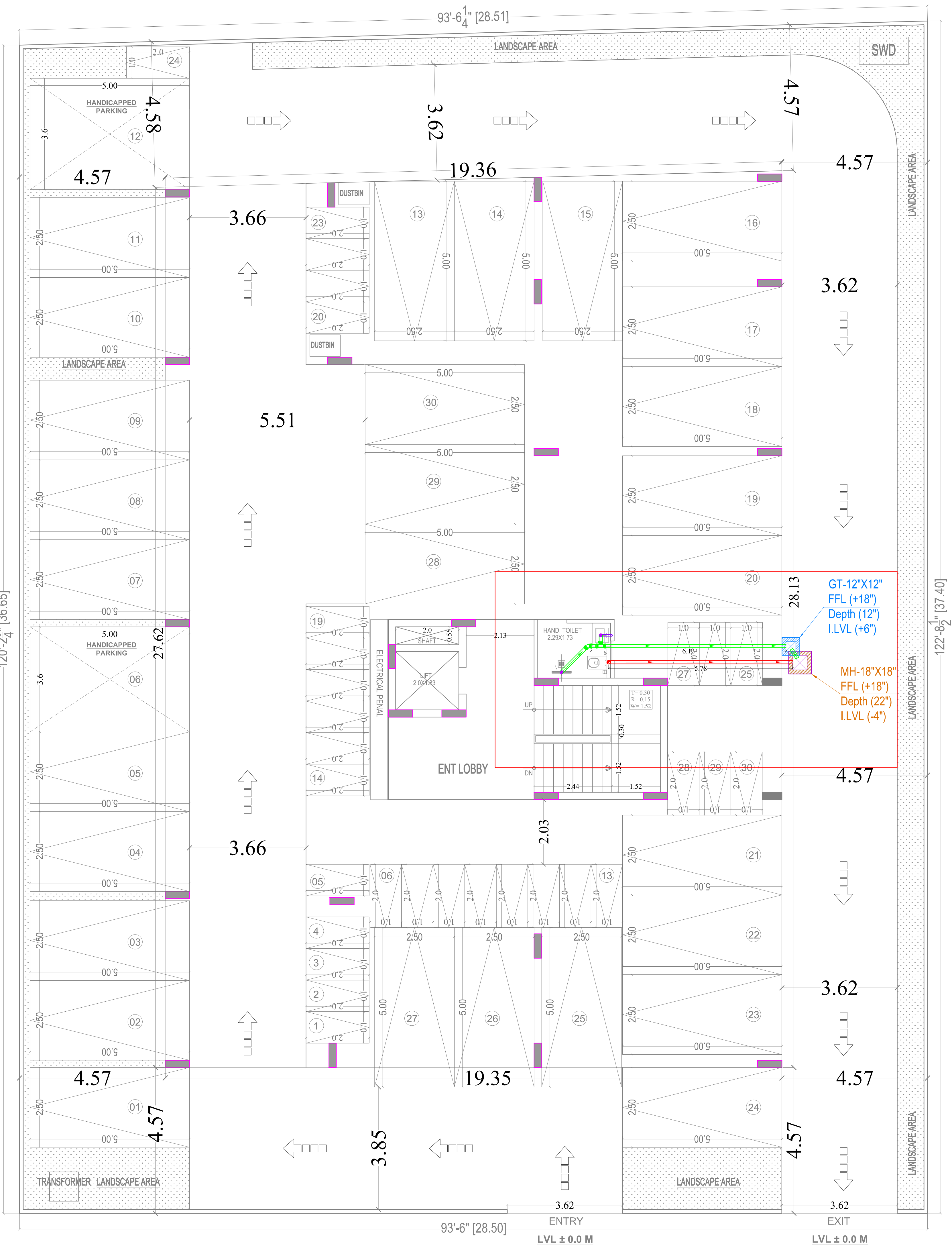
STILT & PARKING FLOOR PLAN
