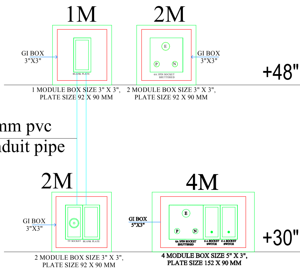
TYPICAL TV WALL ELEVATION PLAN
