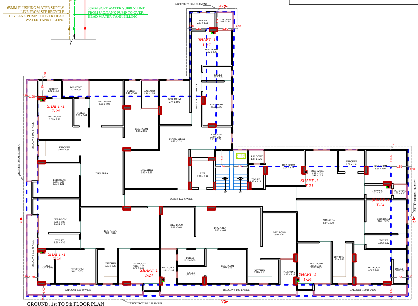
SHAFT MARKING KEY PLAN
