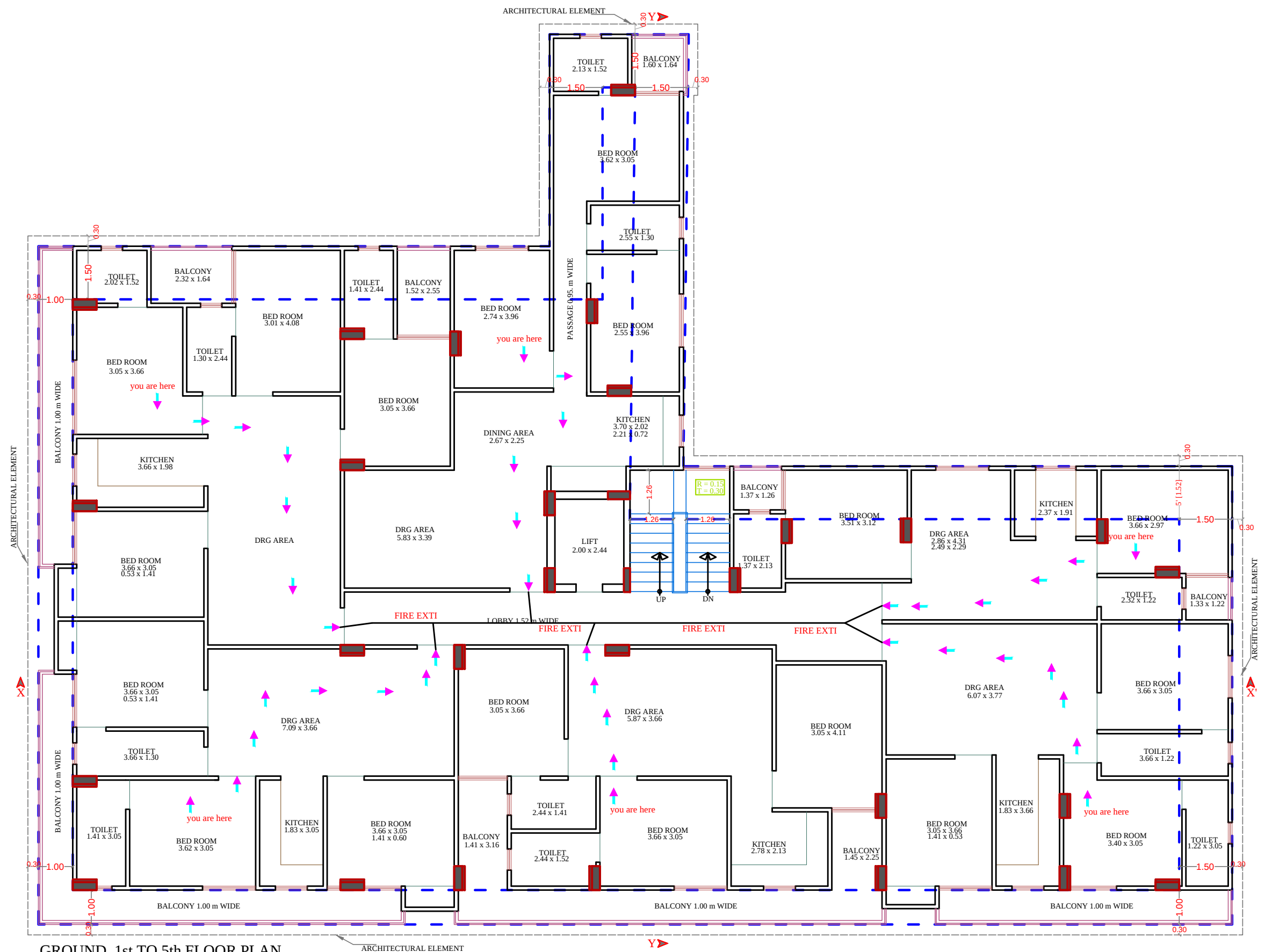
GROUND, 1st TO 5th FLOOR PLAN
