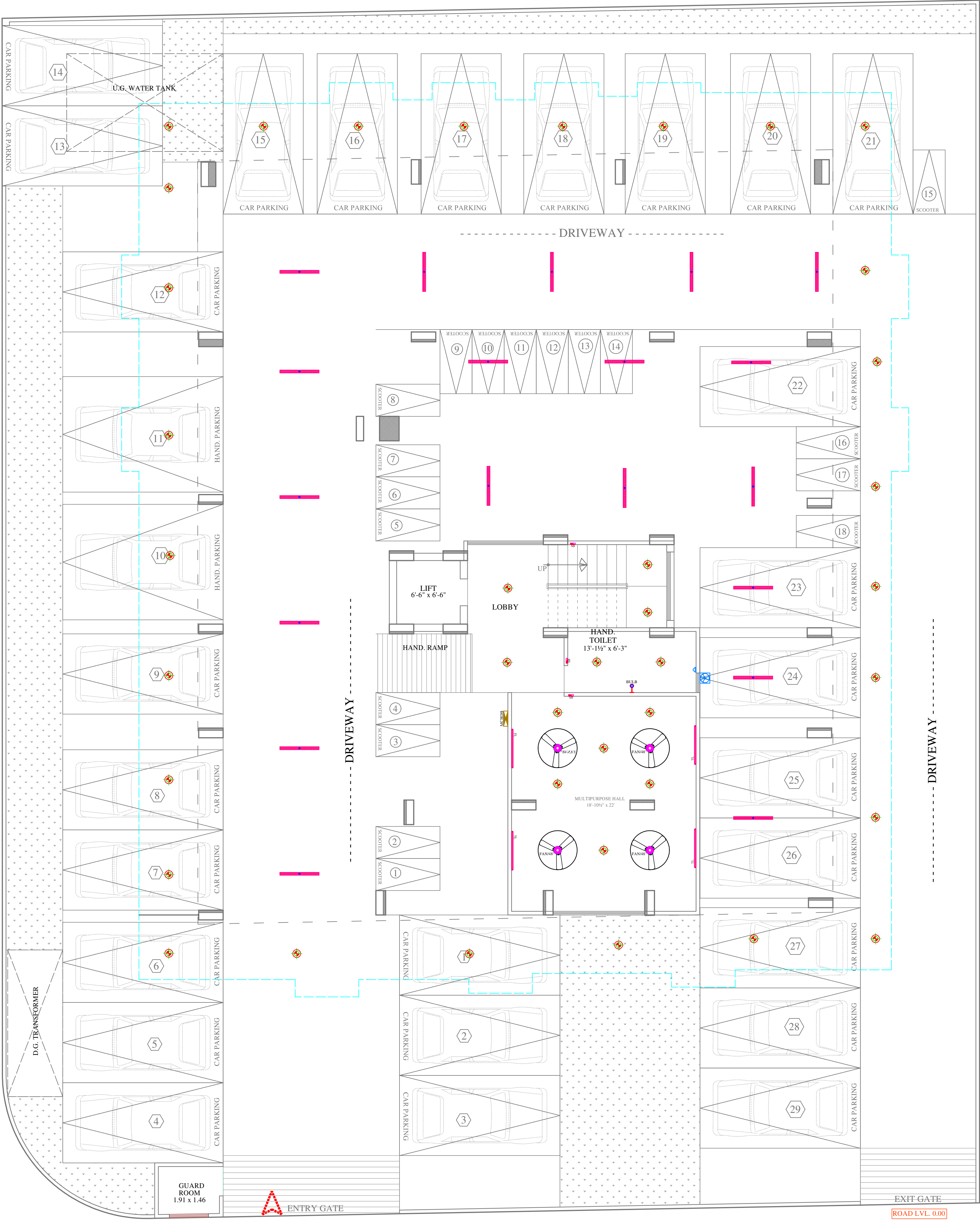
STILT PLAN
