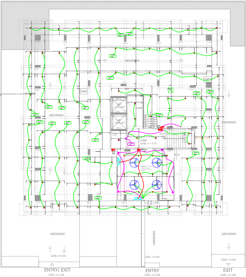
PROPOSED STILT FLOOR ELECTRICAL LAYOUT
