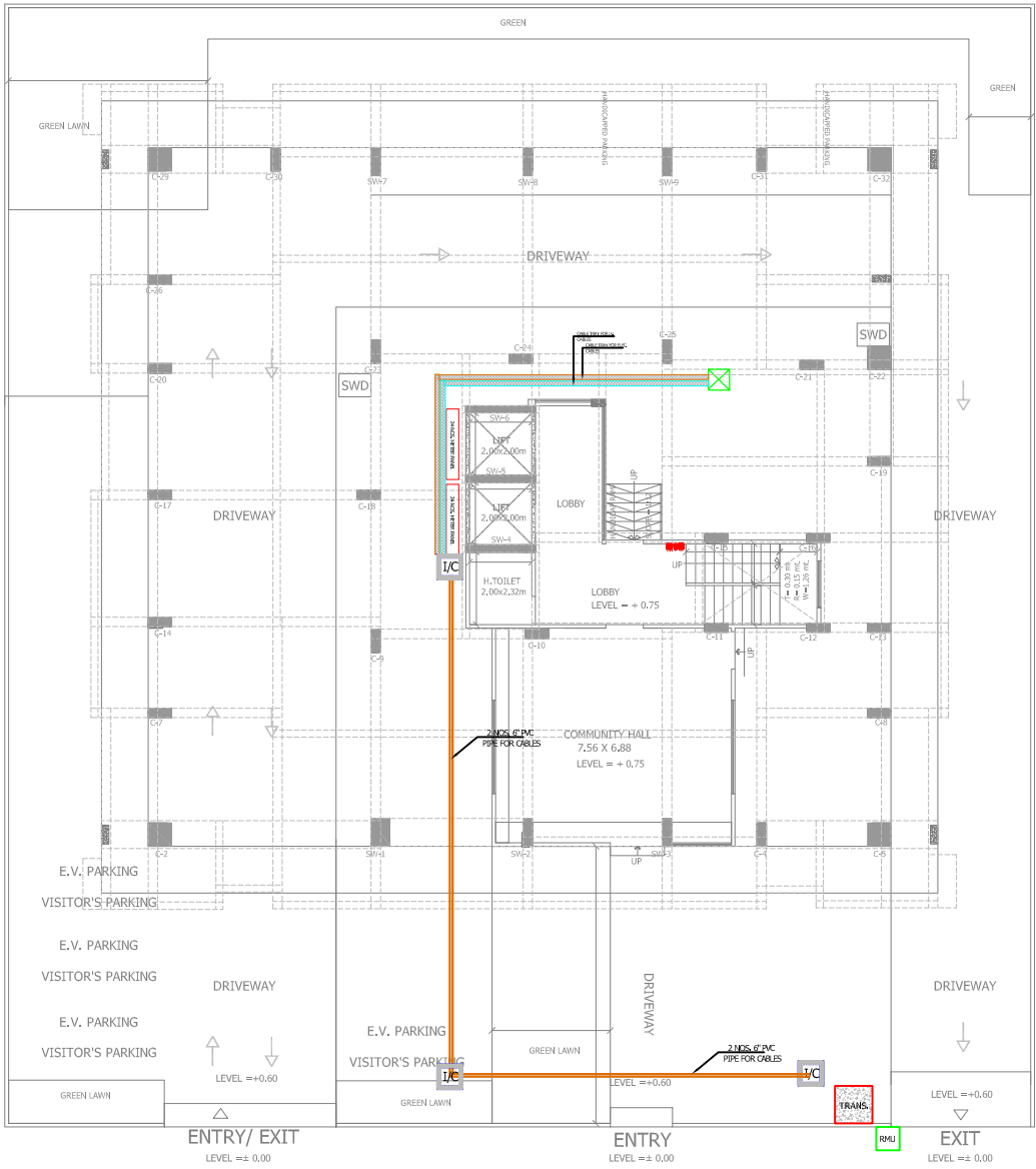
PROPOSED STILT FLOOR ELECTRICAL CABLE ROUTE LAYOUT
