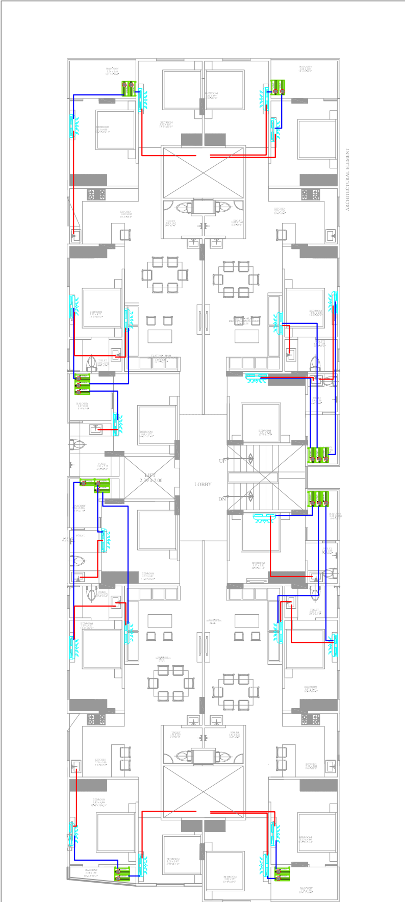
GROUND, 1st TO 5th FLOOR PLAN
