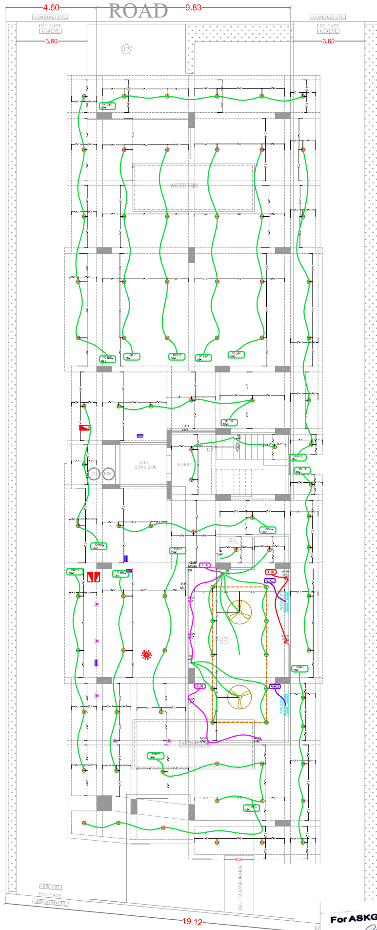
PROPOSED STILT FLOOR ELECTRICAL LAYOUT
