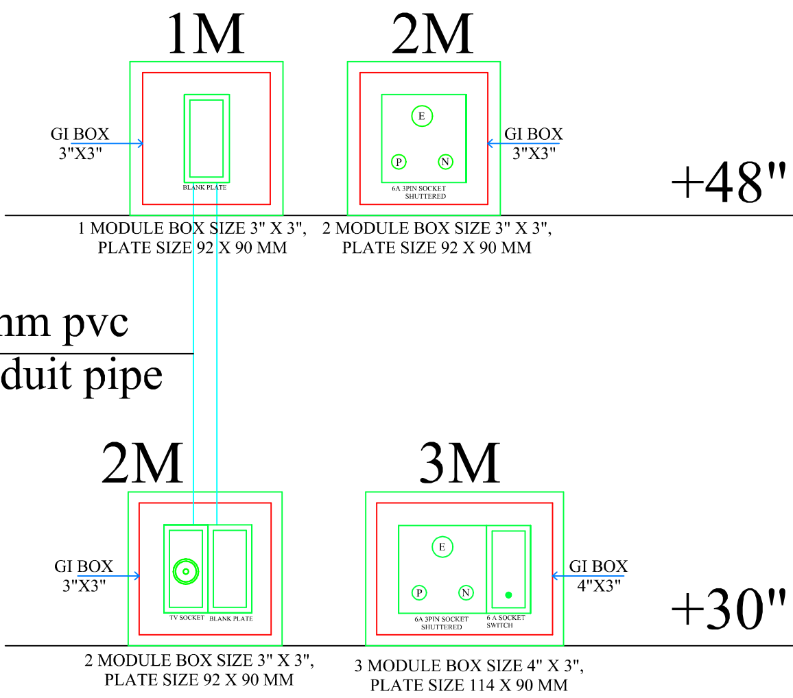
TYPICAL TV WALL ELEVATION PLAN
