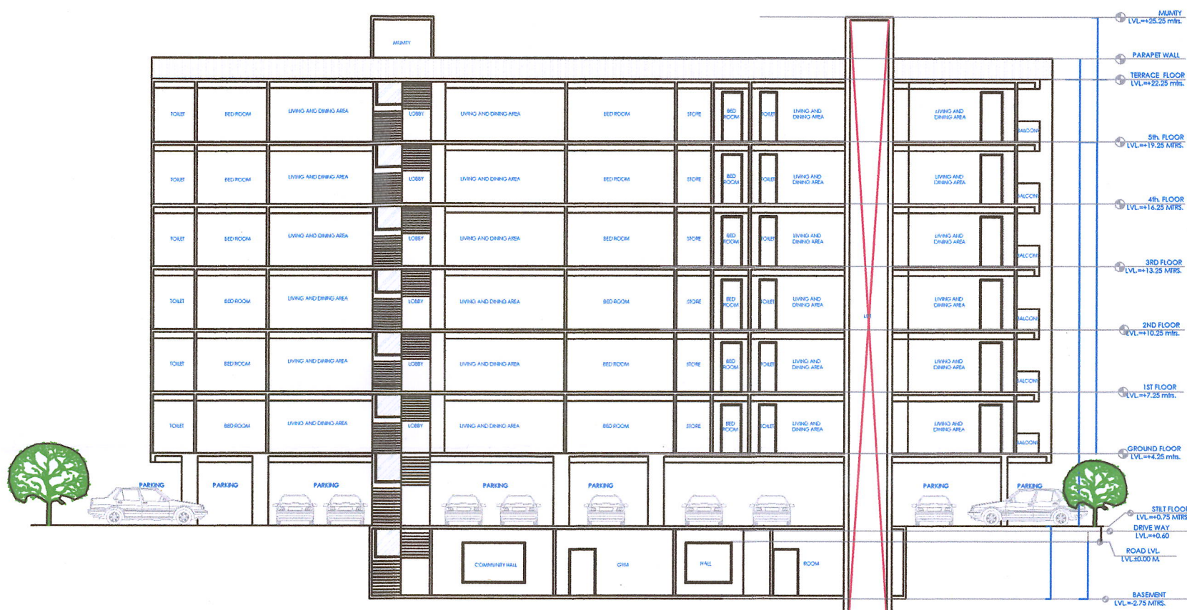
SECTION XX'
