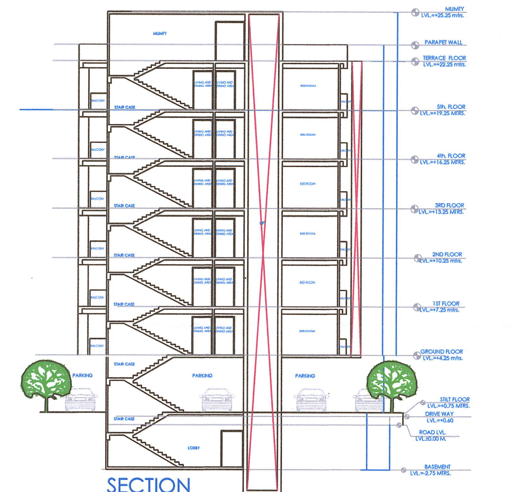
SECTION YY'
